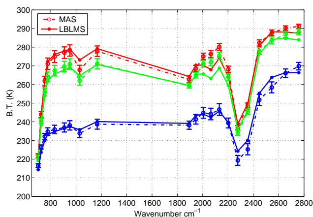
Fig. 14. IR brightness temperature from LBLMS simulated and MAS observed radiance at 20 km. The three colours represent the three sections highlighted in Fig. 10. The vertical bars have same meaning as in Fig. 11.
