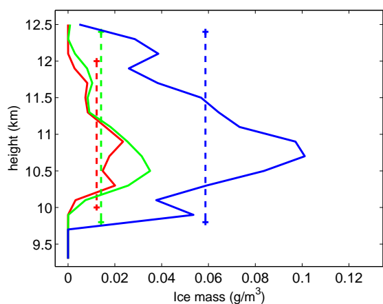
Fig. 17. Average IWC profile, for the LBLMS layering, for Sector 1 (red), 2 (green) and 3 (blue) derived as explained in the text. The vertical dashed lines indicate the profiles adopted for the homogeneous computations.
