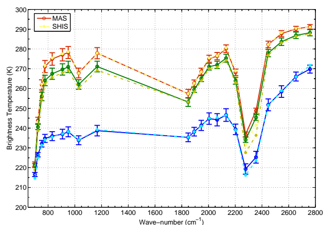
Fig. 11. MAS data averaged over S-HIS nadir FOV and S-HIS data convolved with MAS relative spectral response. The red solid line and yellow dashed refer to Sector 1 (the thin cloud layer); the two green shades are for Sector 2 (medium cloud layer) and the blue lines are for the moderately thick layer of Sector 3. The vertical bars are the one standard deviation of the MAS data around the average values and denote the natural variability as well as radiometric error.
