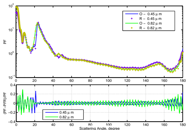
Fig. 2. Upper panel: phase functions in the shortwave at 0.45 \mu\text{m} : Original (PF, blue line) and Reconstructed (PFR, purple crosses); PF at 0.82 \mu\text{m} : Original (green line) and Reconstructed (olive green crosses). Lower panel: fractional difference computed as (\text{PF}-\text{PFR})/\text{PF} .
