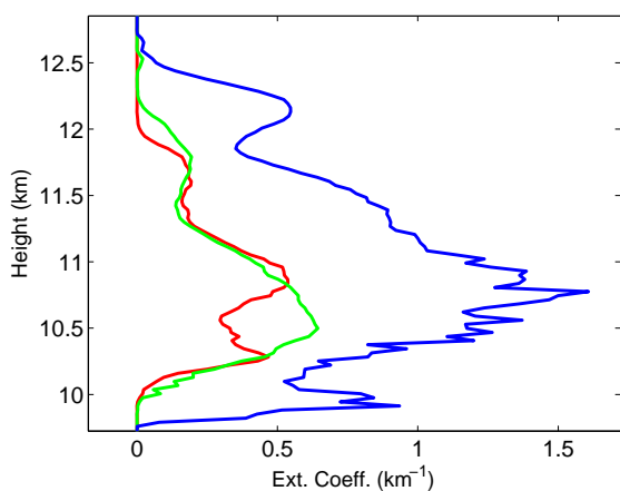
Fig. 16. Average extinction profile for Sector 1 (red), 2 (green) and 3 (blue) derived from CPL.
