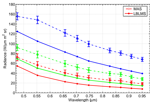
Fig. 12. LBLMS simulations and MAS observations in cloudy conditions – SW range. The three colours represent the three sections highlighted in Fig. 10: red for the thin cloud layer, green for the medium cloud layer and blue for the moderately thick layer. The vertical bars have same meaning as in Fig. 11.
