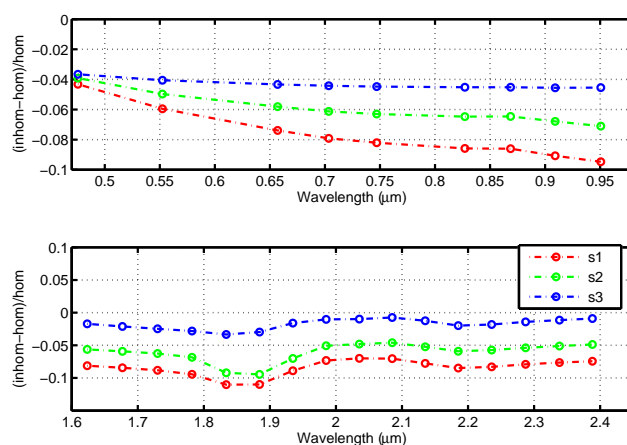
Fig. 18. Fractional difference (\text{Inhom-Hom})/\text{Hom} between the inhomogeneous and the homogeneous cases for the three sectors, in the shortwave (top panel) and near infrared (bottom panel) MAS channels.
