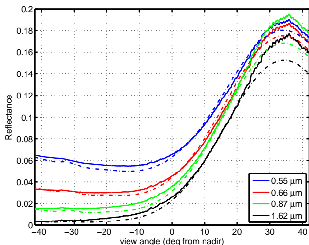
Fig. 7. Reflectance comparison between LBLMS (dashed lines) and MAS (continuous lines) along a MAS scan. Wind speed is 6.5 m/s, aerosol OD at 532 nm 0.07 and pigment concentration 0.07 mg/m 3 .
