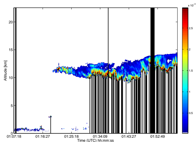
Fig. 9. CPL extinction cross section from 01:07 to 01:54 UTC on the 23 February 2003. Pixels with integrated optical depth smaller than 0.02 are coloured white. Black pixels are those with integrated optical depth greater than 2.98, that is where the signal is saturated, or to pixels for which no CPL measurement is available.
