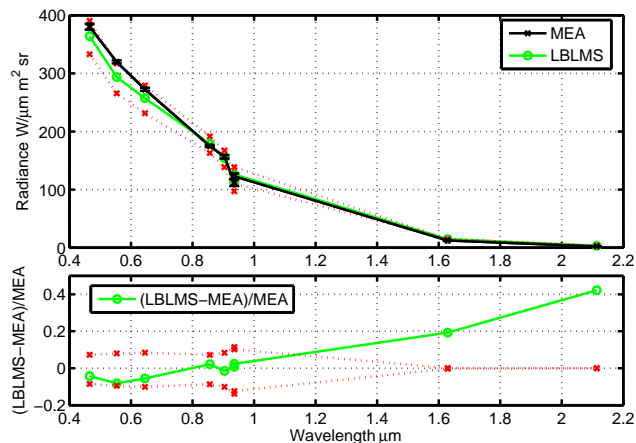
Fig. 25. Same as Fig. 23 but for Area Ci3.
