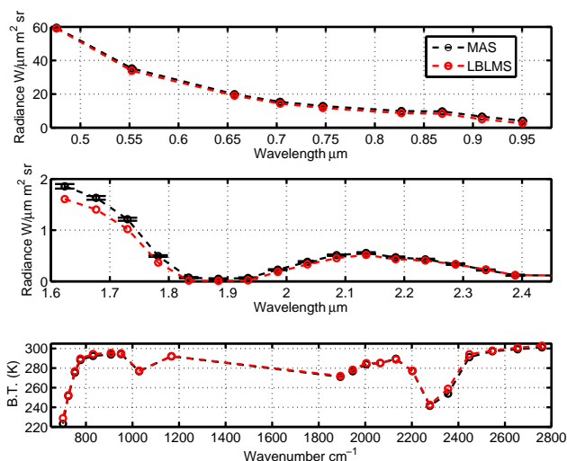
Fig. 4. Comparison of LBLMS simulations and MAS observations at nadir in clear sky conditions. Top and mid panel: comparison of upwelling radiance at 20 km; lower panel: IR brightness temperature.
