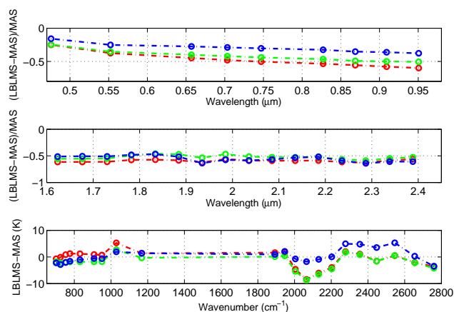
Fig. 15. Differences between LBLMS simulations and MAS observation in cloudy conditions. Top and mid panel: relative radiance errors (\text{LBLMS}-\text{MAS})/\text{MAS} ; lower panel: absolute IR brightness temperature difference (\text{LBLMS}-\text{MAS}, \text{K}) . The three colours represent the three sections highlighted in Fig. 10.
