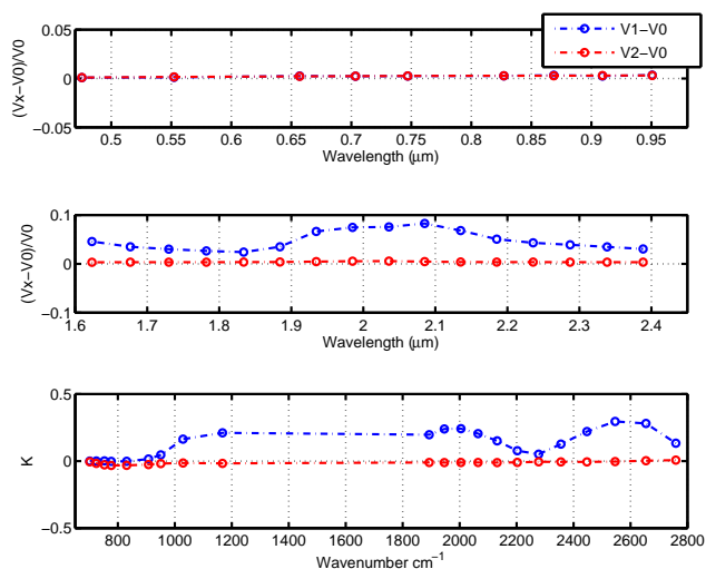
Fig. 19. Comparison between radiance simulated for cases V0, V1, V2 for Sector 1. Top and middle panels: fractional radiance difference with respect to V0; lower panel: brightness temperature difference with respect to V0.
