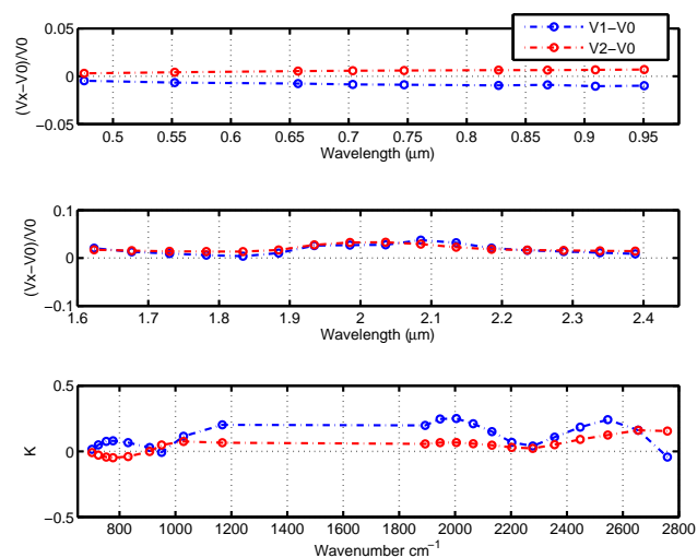
Fig. 20. Same as Fig. 19 but for Sector 2.
