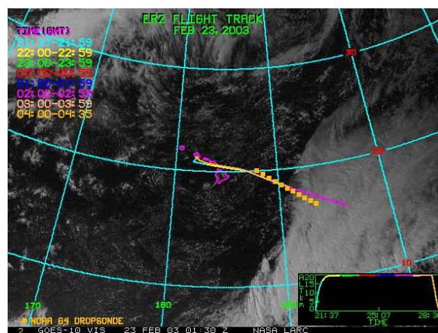
Fig. 1. GOES-10 visible channel image, 23 February 2003. ER-2 route and the drop-sondes positions are shown (from http://www-angler.larc.nasa.gov/thorpex/ ).
