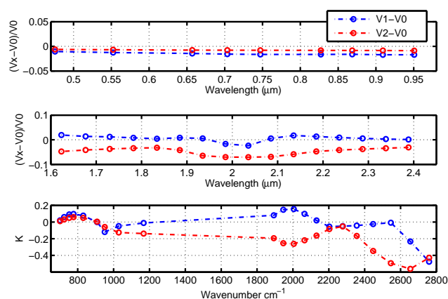
Fig. 21. Same as Fig. 19 but for Sector 3.
