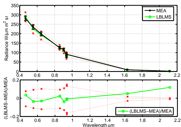
Fig. 24. Same as Fig. 23 but for Area Ci2.
