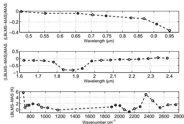
Fig. 5. Differences between LBLMS simulations and MAS observation at nadir in clear sky conditions. Top and mid panel: relative radiance errors (\text{LBLMS}-\text{MAS})/\text{MAS} ; lower panel: absolute IR brightness temperature difference (\text{LBLMS}-\text{MAS}, \text{K}) .
