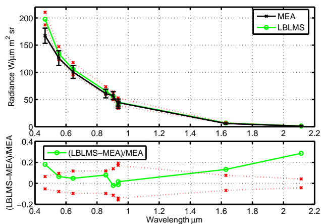
Fig. 23. LBLMS and MODIS radiances for Area Ci1. Upper panel: the black line connects measured MODIS values; the black bars denote the ( 2\sigma ) variability around the mean measured radiance corresponding to same retrieved OT for the area. The green line connects the simulated values (open green circles); the dashed red lines are the radiance computed with OT varied by twice the 1\sigma value given in Table 2 and thus denote the 2\sigma uncertainty level. Lower panel: fractional difference (green line and open circles); the red dashed lines are the 2\sigma uncertainty level.
