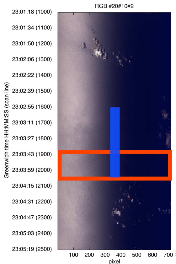
Fig. 3. MAS imagery on Pacific Ocean SE from Hawaiian Islands on 22 February 2003, from 23:01 to 23:05 UTC (roughly 50 km on the ground). The RGB image is obtained from channels 20 ( 2.15 \mu\text{m} ), 10 ( 1.64 \mu\text{m} ), 2 ( 0.55 \mu\text{m} ). The blue line and the red box show the regions chosen for the cross-scan and nadir comparisons.
