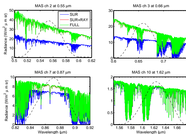
Fig. 6. High resolution spectral radiance in four MAS channels: channel 2 (top left), channel 3 (top right), channel 7 (bottom left) and channel 10 (bottom right). The colour coding is same for all the panels: the blue line labeled SUR is the case when the surface is the sole source function with a molecular atmosphere that only absorbs radiance; the red curve labeled (SUR+RAY) is radiance after molecular scattering is added; the green line (FULL) considers also the presence of aerosol as source function and absorber. The dashed black line is MAS Relative Response Function on a relative scale.
