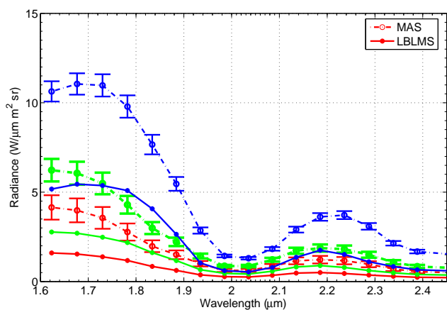
Fig. 13. Same as Fig. 12 but for the NIR spectral range.
