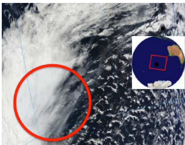
Fig. 22. MODIS RGB image of the scenario used for the comparison with LBLMS. The red circle highlights the cloudy regions used for the test.
