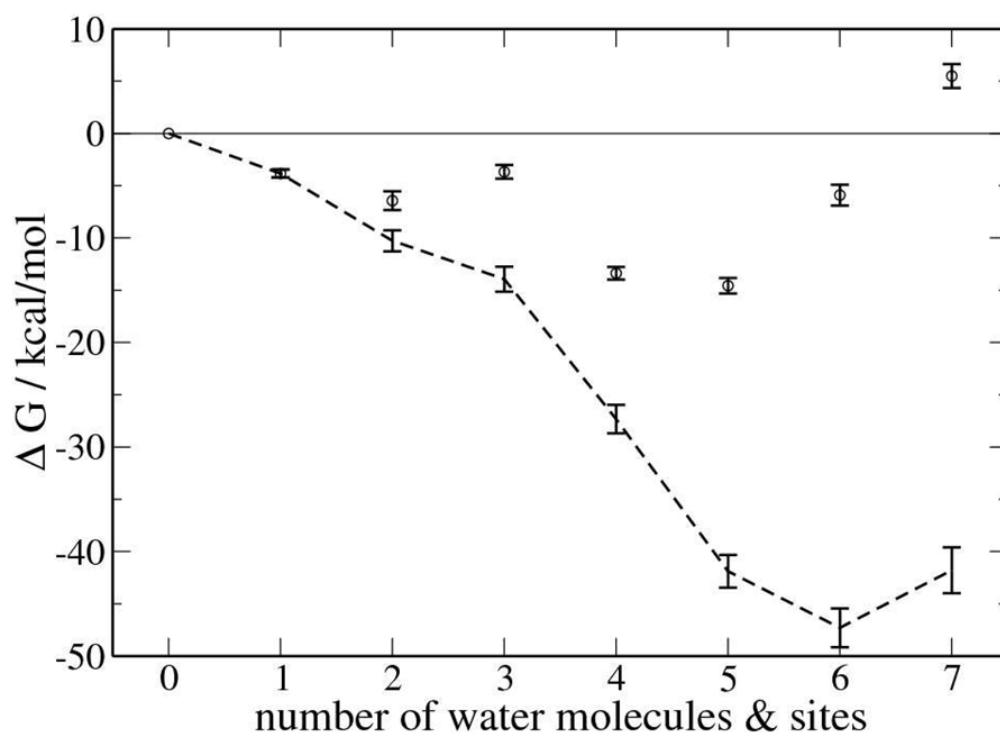
Figure 4. Free energy changes from double-decoupling for the addition of one to seven water molecules in the binding site of the neuraminidase-zanamivir complex. The x-axis shows the number and position of the water molecules, e.g., 3 means three water molecules at sites 1, 2, and 3. Circles denote the free energy change upon addition of each water molecule and the dashed line shows the cumulative free energy change. For clarity, the error bars have been expanded; they represent \pm 5 standard deviations.
