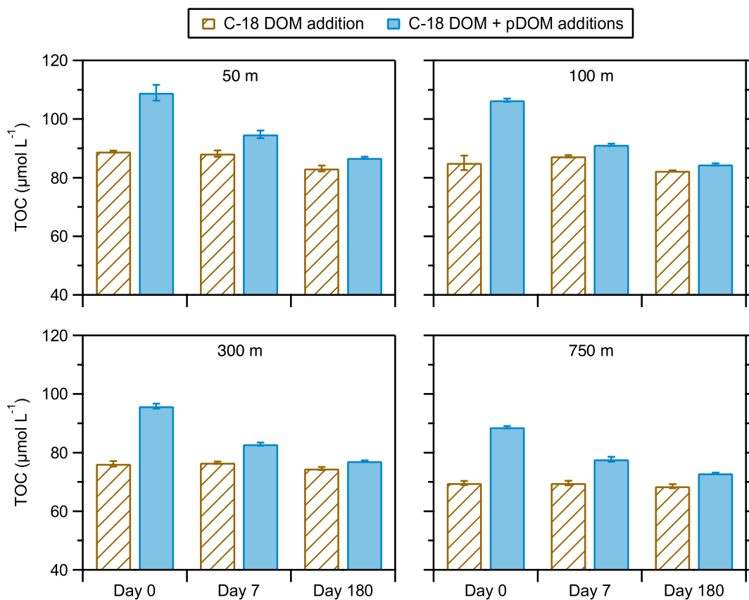
Fig. 4. Changes in concentrations of total organic carbon (TOC) during bioassay experiments with unfiltered waters (50, 100, 300, and 750 m) amended with either C-18 DOM (19–23 \mu\text{mol C L}^{-1} ) or with a combination of C-18 DOM and plankton-derived DOM (39–40 \mu\text{mol C L}^{-1} ). The error bar represents the standard deviation of triplicate experiments. [Color figure can be viewed at wileyonlinelibrary.com ]
