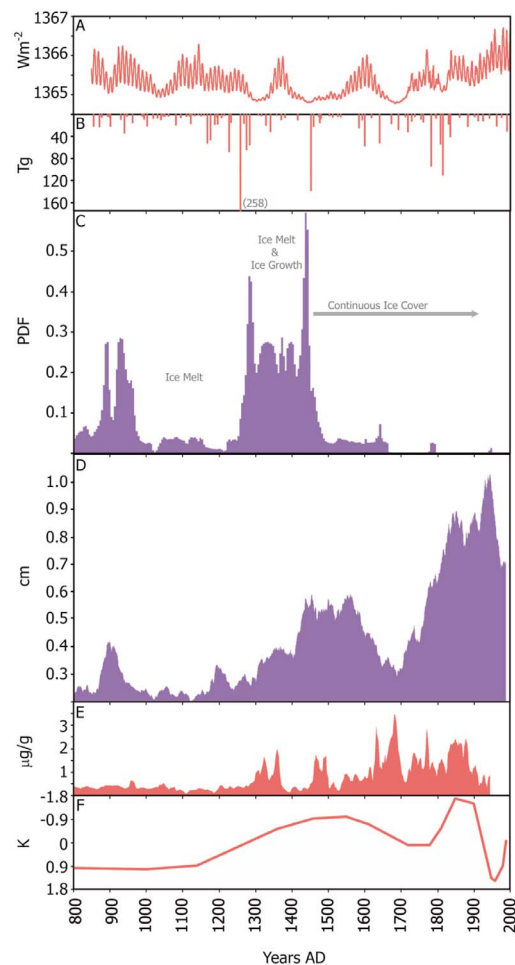
Figure 2. (a) Total solar irradiance (VSK [Schmidt et al., 2011]). (b) Global stratospheric sulfate aerosol loadings [Gao et al., 2008]. (c) Ice cap expansion dates based on a composite of 94 Arctic Canada calibrated ^{14}\text{C} PDFs. (d) 30-year running mean varve thickness in Hvítárvatn sediment core HVT03-2 [Larsen et al., 2011]. (e) Arctic Ocean sea ice recorded in a sediment core on the north Iceland shelf [Massé et al., 2008]; heavy sea ice years correlate with anomalously cold summers across Iceland. (f) Temperature anomalies over southern Greenland (wrt 1881–1980 AD mean) from the borehole temperature inversion at DYE-3 [Dahl-Jensen et al., 1998].
