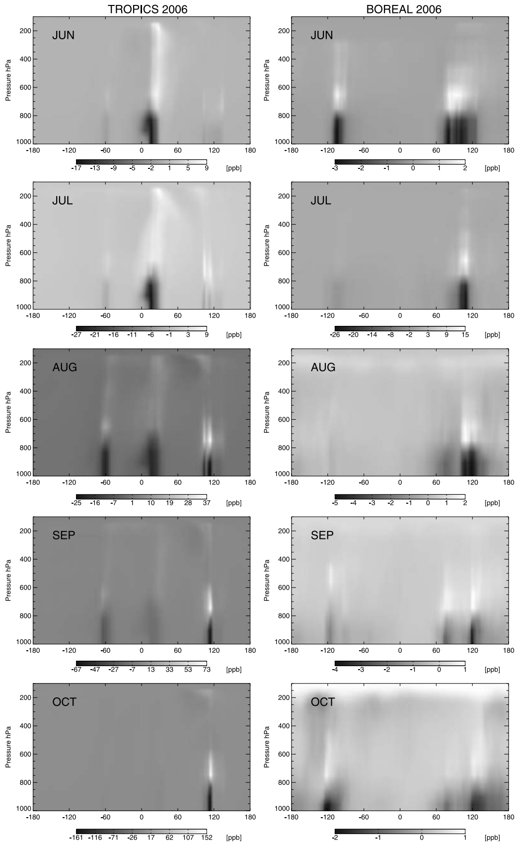
Figure 8. CO concentration differences (ppb) over tropical ( 0^{\circ}\text{S} – 30^{\circ}\text{S} ) and boreal ( 42^{\circ}\text{N} – 67^{\circ}\text{N} ) regions resulting from a GEOS-Chem model run that uses the seasonal average (JJASO 2006) injection heights inferred from TES and MLS measurements (Figure 2) minus a control model run that assumes injection only into the boundary layer.
