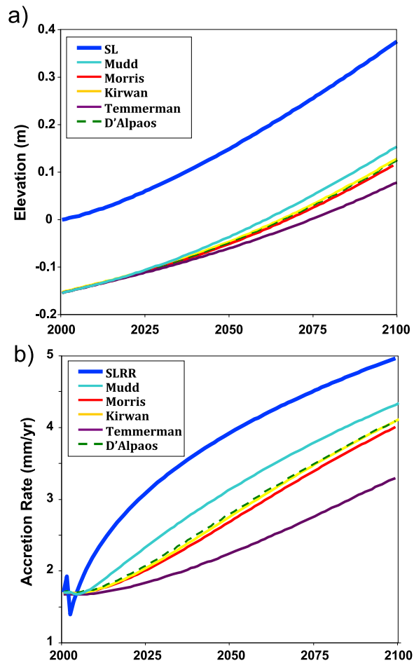
Figure 1. Response of marsh elevation (a) and accretion rate (b) to a conservative sea-level acceleration (IPCC A1B scenario [Bindoff et al., 2007]). Heavy blue line denotes sea level at spring high water (Figure 1a) or the sea-level rise rate (Figure 1b). Elevations reflect the simulated position of the marsh relative to spring high water. Since each model predicts a slightly different initial elevation relative to sea level, we have normalized each model to a common equilibrium elevation at time zero. Since sea-level rise rates tend to exceed accretion rates, marsh elevations adjust to sea-level acceleration by becoming lower relative to sea level (i.e., more inundated) (Figure 1a), which enhances vertical accretion (Figure 1b). (Experimental conditions: spring tidal range = 1 m, suspended sediment concentration = 30 mg/L.)
