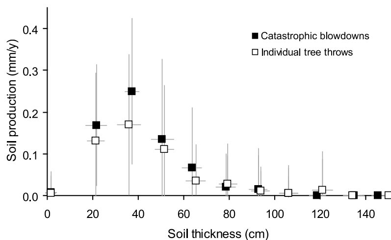
Figure 6. Bedrock erosion rate versus soil thickness from model runs. A humped relationship, with a peak where soil thickness is \sim 35 cm, emerges from the binned and averaged results (error bars = 1\sigma ). Model results suggest that peak soil production rates may be higher in forests where tree throw occurs primarily during large blowdown events.
