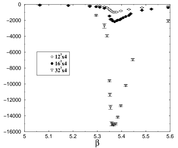
FIG. 2. Behaviour of \rho around the phase transition at various lattice sizes.
