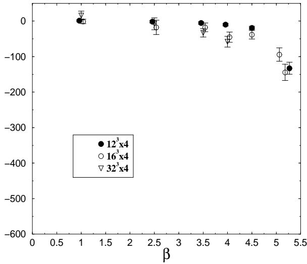
FIG. 4. Strong coupling behaviour of \rho at various lattice sizes and am = 0.1335 .
