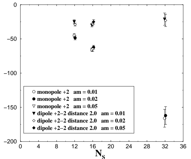
FIG. 3. Weak coupling behaviour of \rho at various lattice sizes.
