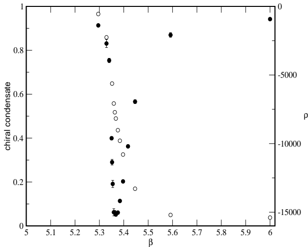
FIG. 1. Chiral condensate (open circles) and \rho (filled circles) on the 32^3 \times 4 lattice.
