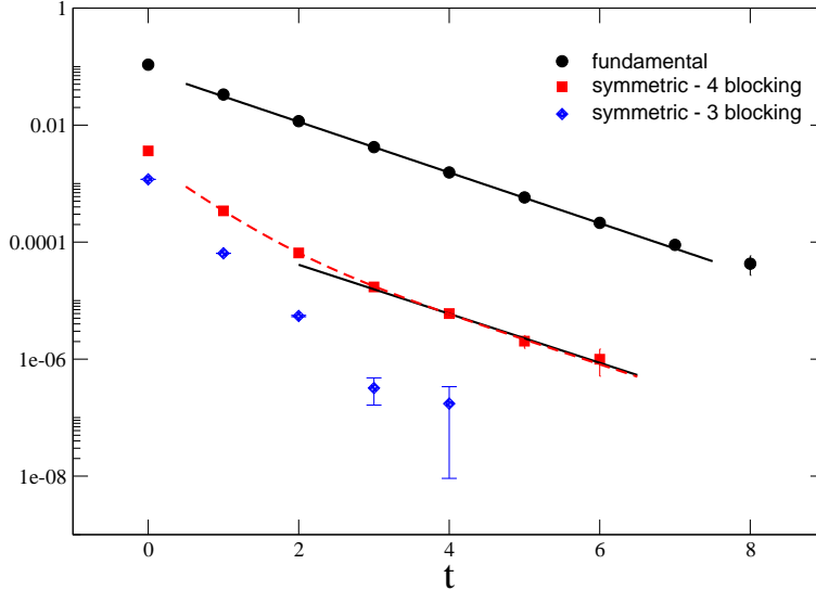
Figure 1: Correlator data for the fundamental (circles) and rank-2 symmetric (squares) representations, with L = 16 , as a function of the temporal distance t . The top solid line is a hyperbolic cosine fit to data with t \geq 3 , leading to an estimate of m_1 ; the bottom solid line is a hyperbolic cosine with the same exponent, which is well supported by the symmetric representation data for t \geq 3 . The dashed line represents a fit using the two-exponent Ansatz (6). Data from the rank-2 symmetric representation at one less blocking step is shown in diamonds.
