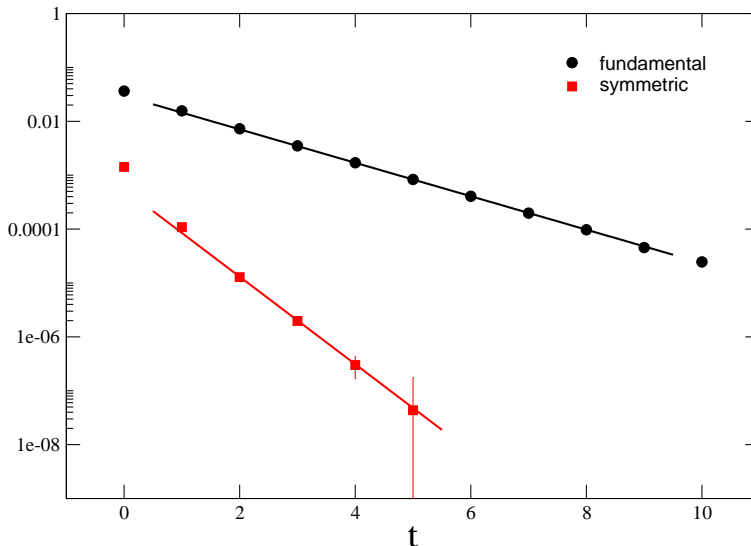
Figure 2: Correlator data for the fundamental (circles) and symmetric (squares) representations, with L = 12 , as a function of the temporal distance t . Solid lines are exponential fits to data with t \geq 3 , leading to markedly different values of m_k .
