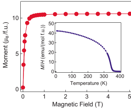
FIG. 2. (Color online) Isothermal magnetization of \text{BiCu}_{2.4}\text{Mn}_{4.6}\text{O}_{12} at 5 K and the temperature dependence of the dc magnetic susceptibility in a magnetic field of 0.1 T (inset), both assuming stoichiometric composition. The saturation magnetization was corrected to be 12.1 \mu_B/\text{f.u.} considering the off-stoichiometry, as described in the text.
