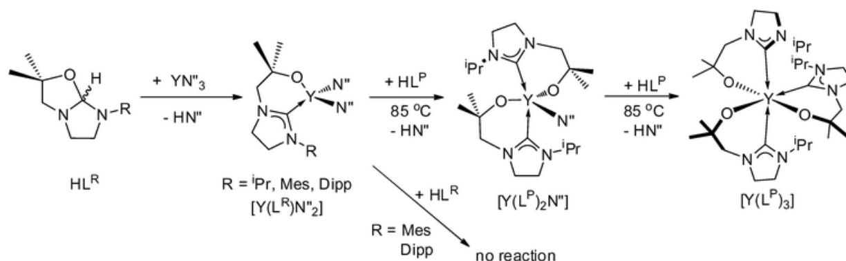
Scheme 1. Sequential NMR scale syntheses of Y^{III} -NHC complexes.
