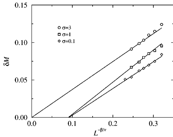
FIG. 3. Standard deviation, \delta M_L , of the ordering operator, \mathcal{M} , as a function of L^{-\beta/\nu} , where L is the simulation box dimension, and \beta and \nu are the order parameter and correlation decay exponents, respectively: \sigma=3 (circles); \sigma=1 (squares); \sigma=0.1 (diamonds). The lines are linear fits to the results for L/d \geq 12 in each case.
