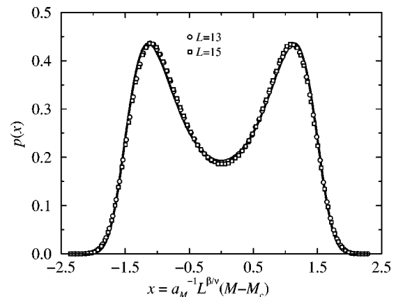
FIG. 6. Critical ordering operator distributions for \sigma=1 : p_L(x) for L/d=13 (circles) and L/d=15 (squares); limiting Ising distribution, p_{Is}^*(x) , from Ref. 28 (solid line).
