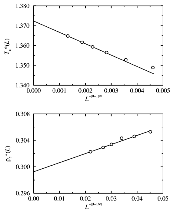
FIG. 8. Extrapolation of the critical temperature (top) and critical density (bottom) for \sigma=1 to the limit L^{-1}\rightarrow 0 . The solid lines are extrapolations of the results for the three largest system sizes ( L/d\geq 12 ).
