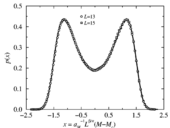
FIG. 2. Critical ordering operator distributions for \sigma=3 : p_L(x) for L/d=13 (circles) and L/d=15 (squares); limiting Ising distribution, p_{Is}^*(x) , from Ref. 28 (solid line).
