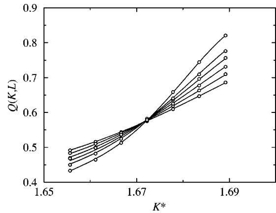
FIG. 5. Cumulant ratio, Q(K,L) = \langle \mathcal{M}^2 \rangle_{K,L}^2 / \langle \mathcal{M}^4 \rangle_{K,L} , as a function of reduced temperature, K^* , for \sigma=3 and, from top right to bottom right, L/d=15 , L/d=13 , L/d=12 , L/d=11 , L/d=10 , and L/d=9 . The solid lines represent a fit to the simulation data using Eq. (9).
