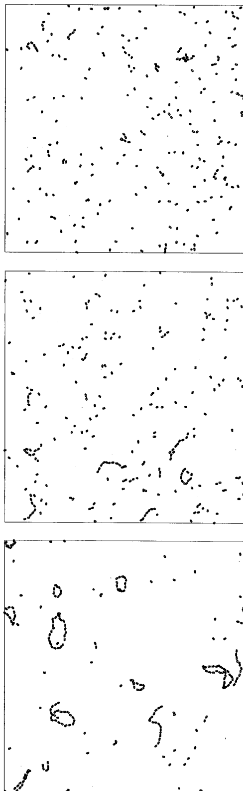
FIG. 3. The structure of a low density ( \rho^* = 0.001 ) dipolar fluid modeled using BD with different parameters describing the coupling to the “solvent bath.” Results are shown for the following parameters: (top) \Theta^* = 4 , D^* = 0.04 ; (middle) \Theta^* = 400 , D^* = 4.0 ; (bottom) \Theta^* = 4000 , D^* = 40 .
