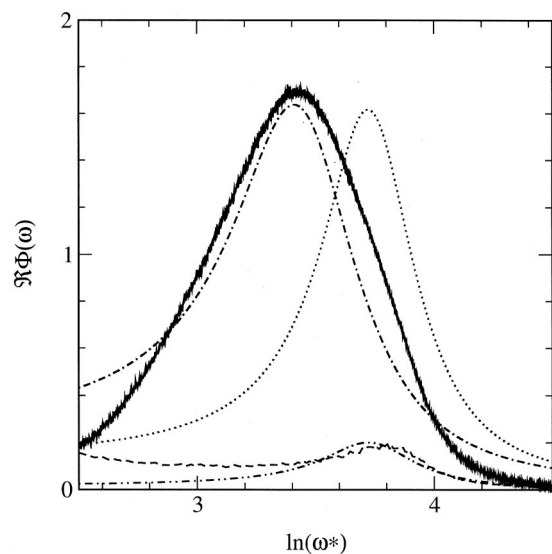
FIG. 5. Comparison of theory and BD simulation results ( \rho^* = 0.06 , D^* = 0.04 , \Theta^* = 4 ) for the real parts of \Phi_S(\omega) and \Phi_M(\omega) . The solid and dashed curves are BD results for \Re\Phi_S(\omega) and \Re\Phi_M(\omega) , respectively. The remaining curves represent the following model calculations: dotted, \tau_V^* = 0.1 , \langle \gamma^2 \rangle = 0.0645 , \omega_0^* = 41 ; dashed-dotted, \tau_V^* = 0.1 , \langle \gamma^2 \rangle = 0.0645 , \omega_0^* = 30 ; dashed-dotted-dotted, \tau_V^* = 0.1 , \langle \gamma'^2 \rangle = 0.008 , \omega_0^* = 45 .
