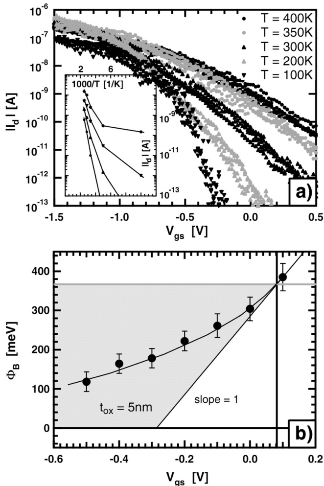
FIG. 13. (a) I_{V_g} characteristics at different temperatures for a CNTFET with t_{ox} = 5\text{ nm} taken at V_d = 0.5\text{ V} . The inset displays Arrhenius plots for V_g values of -0.5 , -0.3 , -0.1 , and +0.1\text{ V} (from the top to bottom). (b) Schottky barrier height for the same device as a function of V_g . Reprinted with permission from J. Appenzeller, M. Radosaveljević, J. Knoch, and P. Avouris, Phys. Rev. Lett. 92 , 048301 (2004). Copyright © 2004, American Physical Society.
