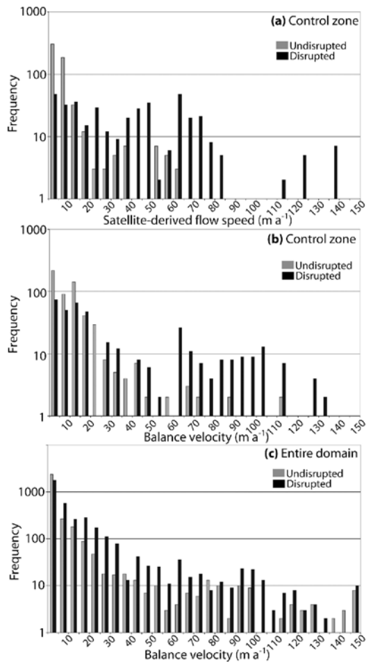
Figure 4. Histograms of internal layering characteristics versus ice flow speeds. Datapoints along each RES flight track were characterized as exhibiting primarily undisturbed (gray columns) or disrupted (black columns) internal layering, and are here plotted against (a) satellite-derived ice-flow speeds, only available in the control zone; (b) balance velocities only in the control zone; and (c) balance velocities across the entire study domain. In all three cases, disrupted internal layering predominates over undisturbed layering at higher ice-flow speeds.
