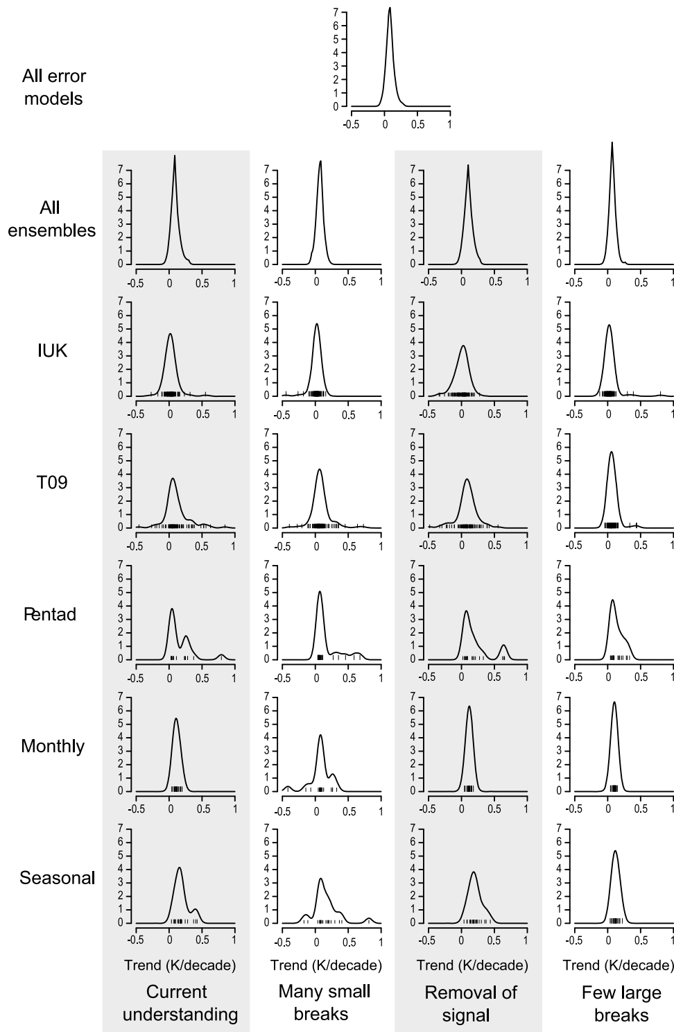
Figure 11. Tropical TLT trends 1979–2003. For each ensemble, the real-world adjusted trends have been scaled by the known errors in each error model, and the resulting ensemble of trends are shown as a rug plot and as a PDF generated by smoothing the ensemble with a Gaussian kernel density estimator. The “All ensembles” row shows the PDFs from the combined ensemble estimates, and the top plot is the mean over the four error models.
