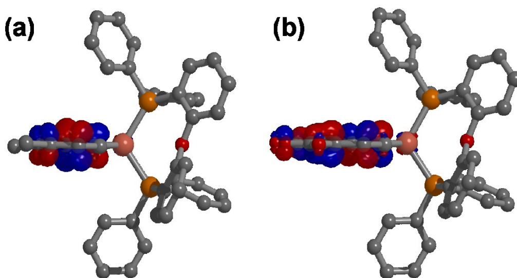
Figure 6. Isosurface images generated from DFT calculations of (a) LUMO for 4 ; (b) LUMO for 5
