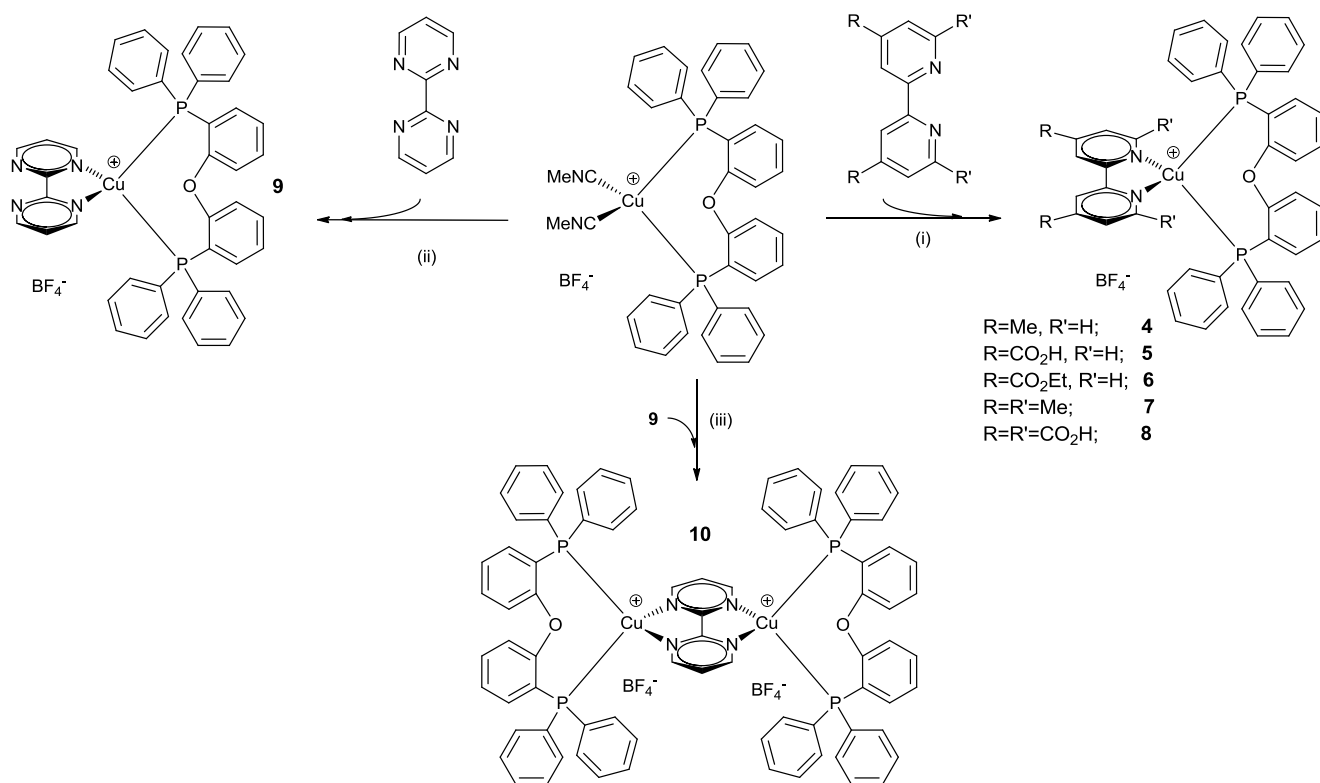
Figure 2. Synthetic Reaction Scheme for Heteroleptic Complexes reported in this work. (i) 4, 5, 6, 8 acetone; 7 anhydrous acetonitrile (ii) DCM (iii) acetone.
