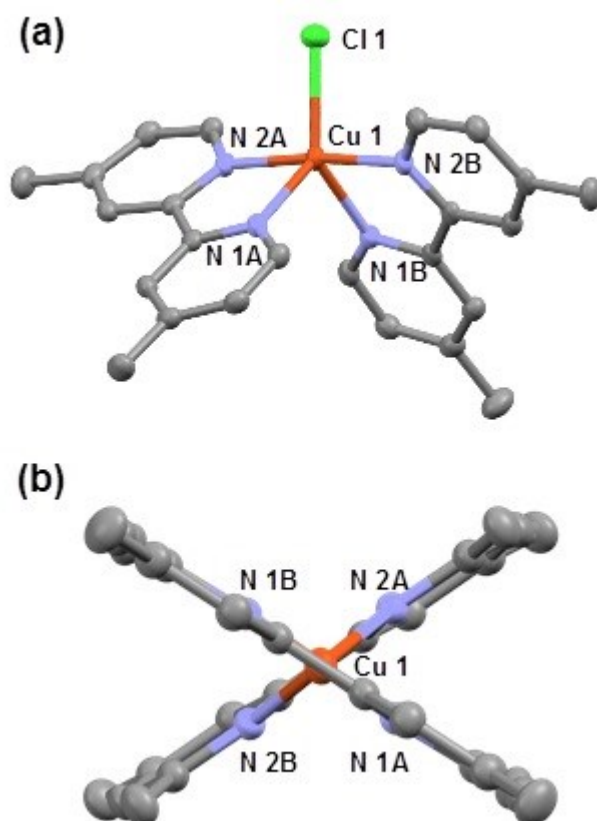
Figure 3. Mercury plots of (a) [\text{Cu}(\text{dmbpy})_2\text{Cl}][\text{BF}_4] ; and (b) 1 . Thermal ellipsoids are drawn at the 50% probability level. [\text{BF}_4] counter ion omitted for clarity. Selected bond lengths and bond angles for
