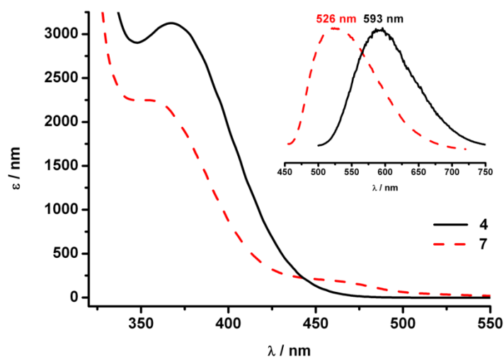
Figure 7. Absorbance and Emission Spectra for heteroleptic complexes 4 and 7 . Absorbance spectrum carried out in MeCN; Fluorescence emission spectrum recorded in a rigid matrix of EtOH.
