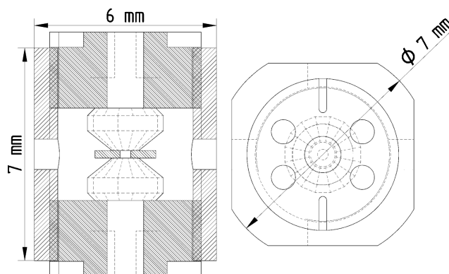
FIG. 1. Drawings of the TM-DAC with key dimensions.
