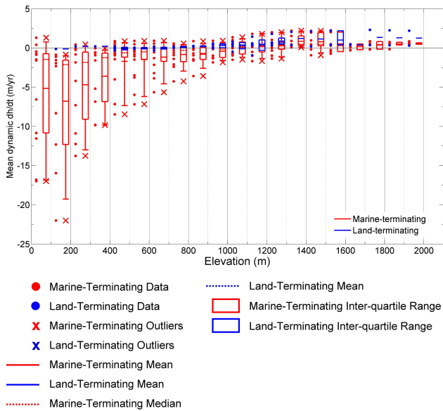
Fig. 6. The magnitude of differences between observed thinning and thinning calculated by a PDD model for all outlet glaciers shown in Fig. 1 and for all years we have data (i.e. not just 1993 to 1998 and 1998 to 2006).
