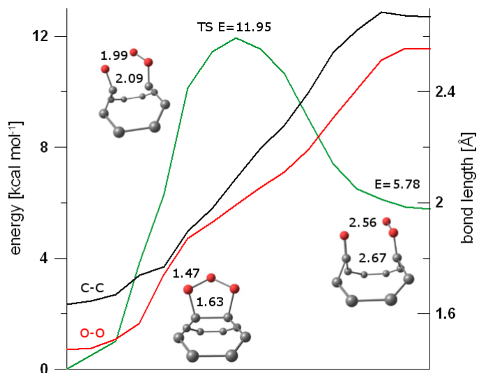
Figure 5 Calculated energy profile (in green) for the a,b\text{-C}_{70}\text{O}_3 ring opening reaction, leading to the product a,b\text{-C}_{70}\text{O}_3^{(\text{dis})}(\text{I}) . Changes in bond lengths observed for C-C and O-O are given in black and red, respectively.
