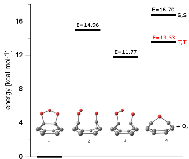
Figure 8 Characteristic points on the decomposition pathway of c,c -C 70 O 3 . Structures 1 and 3 represent minima, 2 is a transition state on the S 0 PES and 4 is a minimum on the T 1 PES of c,c -C 70 O.
