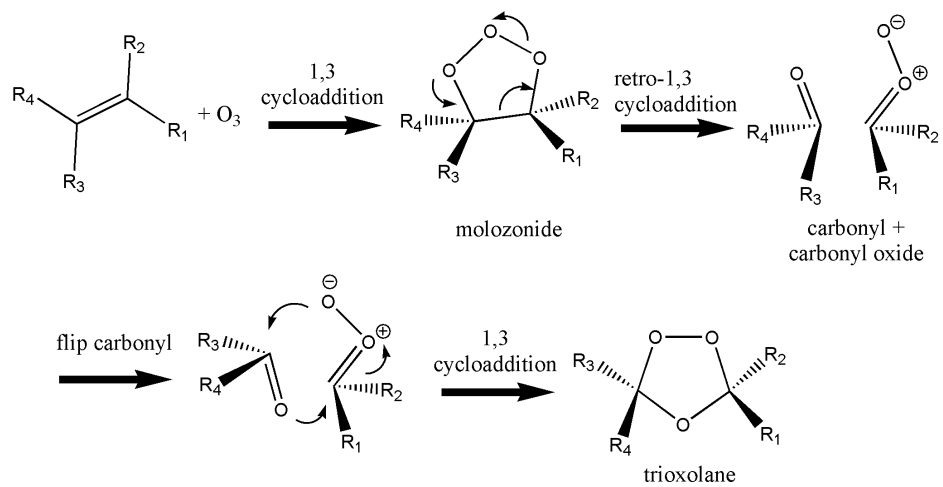
Scheme 1 Criegee's mechanism of ozonolysis.
