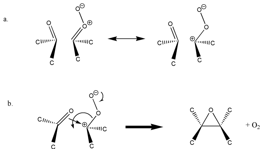
Scheme 2 (a) Proposed resonant structures for the products of the ozonide ring opening reaction, and (b) a possible mechanism for the formation of the closed oxide structure.
