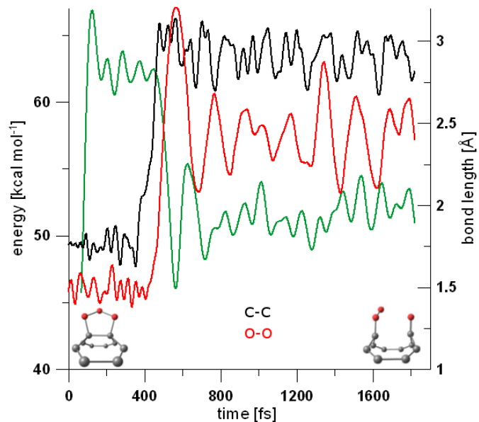
Figure 3 Selected parameters obtained from a section of the MD run performed for e,e -C 70 O 3 . The bond lengths C-C (black) and O-O (red) as well as the potential energy (green) are depicted versus simulation time.
