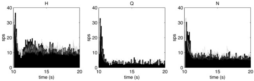
Figure 10: The estimated firing rate in spikes per second (sps) from five randomly selected trials (gray) in the online data, overlaying the PSTH (black) of responses to the respective stimuli, H (HCl), Q (quinine) and N (NaCl) in cell 9. The approximate firing rate is computed as p(y_k = 1|x_k, \theta_k)/\Delta .
