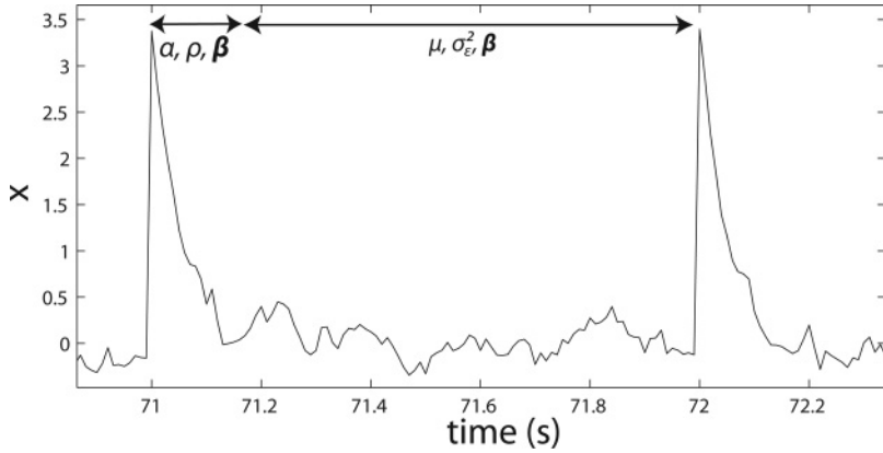
Figure 3: Selective updating of parameter estimates in an online framework is carried out in accordance with the areas where the state bears most information about the relevant parameters of interest. In this case, the narrow stretch close to an input spike bears a lot of information on the state decay factor \rho and the input gain \alpha . The noise parameters \mu and \sigma_\epsilon^2 are more evident in regions of no input.
