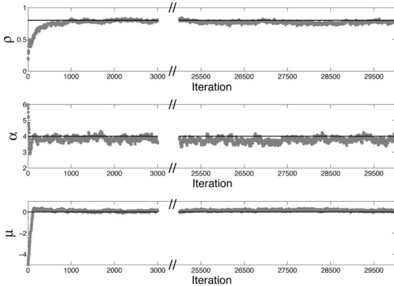
Figure 11: The trajectory of the Gibbs sampler for the unknown parameters \rho , \alpha , and \mu . The solid level line denotes the true parameter value.
