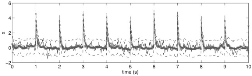
Figure 1: True state (continuous unmarked line) and mean estimated state (marked line) as given by the batch VB algorithm in the final iteration. The true state lies consistently within the 99% confidence intervals (dashed line).
