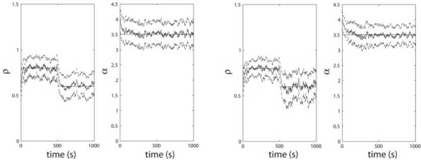
Figure 5: Online tracking of a sudden change in the true parameter (level black line) \rho at time t = 500 s. In this example, \mu and \beta were assumed constant and known from previous offline analysis of the system. The 99% confidence intervals (outer traces) are seen to enclose the true value on the filter reaching a steady behavior for both the (left) VB filter and (right) particle filter with 5000 particles.
