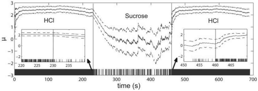
Figure 7: Tracking the mean (solid) and corresponding 99% intervals (dashed) of \mu indicating a change in stimulus from HCl to sucrose and back to HCl in cell 9. The parameter change is indicative of a change in the spike train pattern (inset) when the stimulus is changed. The solid vertical lines indicate where the change in applied chemical stimulus took place. For this trial, \alpha was fixed to 0.1.
