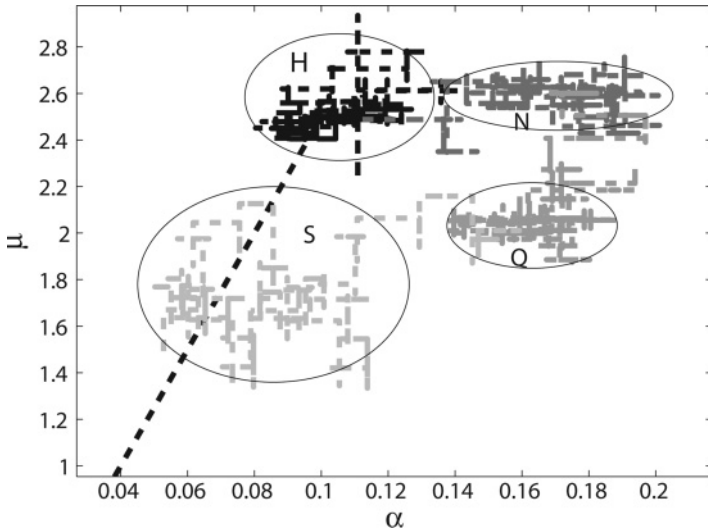
Figure 9: Cell 11—temporal progression of the estimated mean of \alpha and \mu indicating a change of stimulus from (in order of decreasing contrast) HCl (H) to NaCl (N) to quinine (Q) to sucrose (S). From this chart, it is evident that \alpha or \mu on their own cannot capture the difference in response to the different tastants. The ellipses define arbitrarily chosen classification boundaries.
