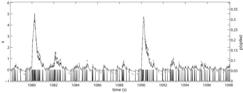
Figure 6: A 20 s segment of training data taken from the cell 9 response to NaCl. The time duration shown spans across two trials with the rinsing and phase 1 periods removed. The estimated state (dashed line) and probability of a spike occurring (solid line) are seen to be indicative of the frequency of spike events (shown on the bottom axis).
