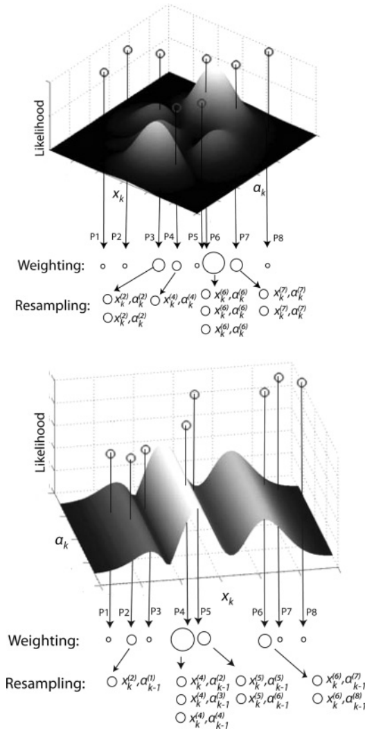
Figure 4: (Top) The likelihood function is used to appropriately weight the particles ( P\# ) representing the posterior distribution, which are then resampled into N particles of equal weight. (Bottom) In this case, the likelihood is practically independent of \alpha_k , and thus the weighing and resampling steps depend solely on the x_k component of the particles. In order to maintain the posterior distribution with fewer particles than would be necessary otherwise, the prior particle parameter set is redistributed after resampling, with equal weight among the resampled particles. The figures (top) and (bottom) correspond to the two areas marked in Figure 3, respectively (likelihood surfaces shown are for illustration only and do not represent actual surfaces).
