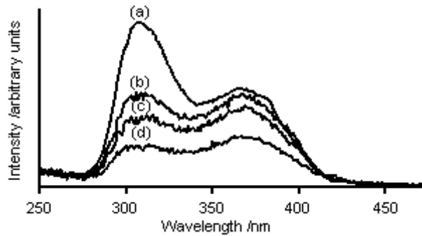
Figure 3. Excitation spectra of the GPA(T) duplex, detected at (a) 440 nm, (b) 460 nm, (c) 470 nm and (d) 490 nm.
