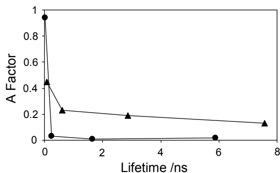
Figure 3. Graphical representation of the decay parameters for the AP1 duplex when free in solution (circles) and in ternary complex with M.EcoRV and cofactor AdoHcy (triangles).
