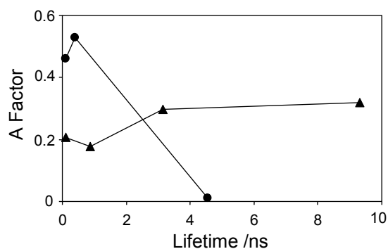
Figure 2. Graphical representation of the decay parameters for the AP2 duplex when free in solution (circles) and in ternary complex with M.EcoRV and cofactor AdoHcy (triangles).
