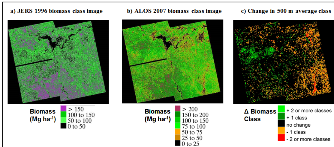
Figure 7: Biomass class images produced using a) JERS HH 1996 data and b) ALOS HV 2007 data, using scales with the size of biomass classes based on RMSE error values, with broader classes for the JERS HH 1996 data than the ALOS HV 2007 data; and c) change in 500 m average class (JERS class image subtracted from ALOS class image) for the two images (using the broader JERS classes).
