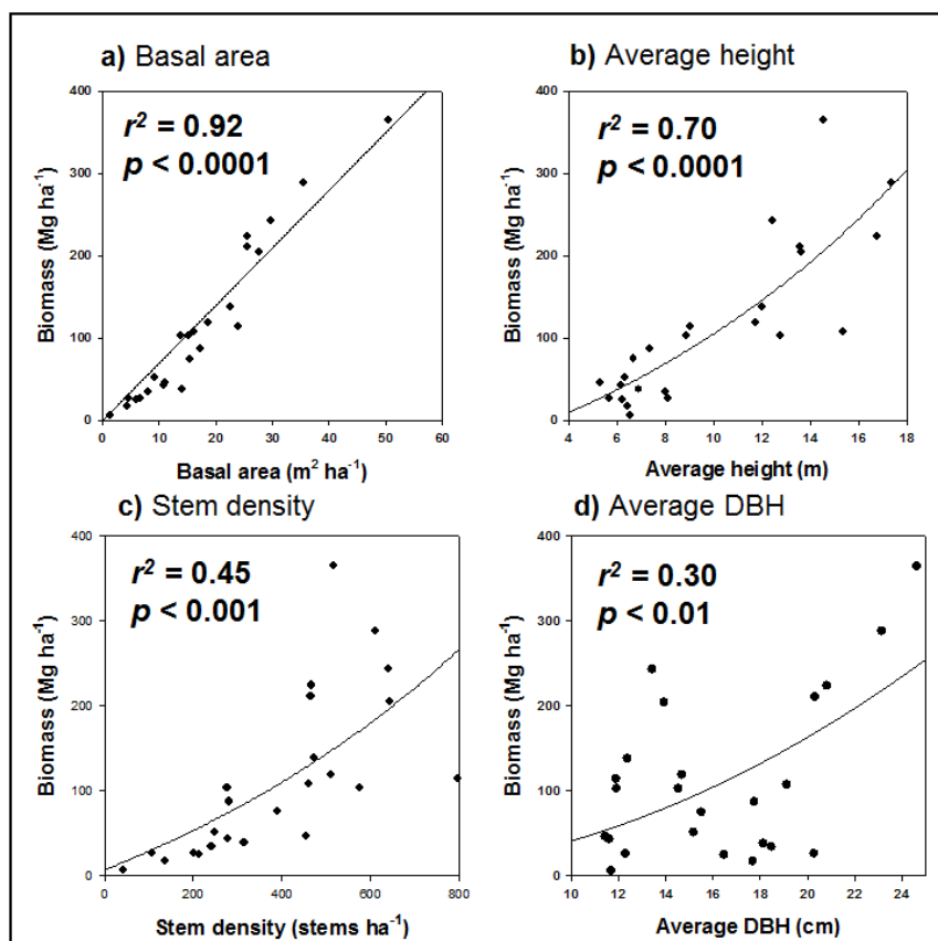
Figure 2: Biomass values for the field plots against a) basal area, b), average height, c) stem density, and d) average DBH. The fit for a is linear, for b, c and d quadratic.
