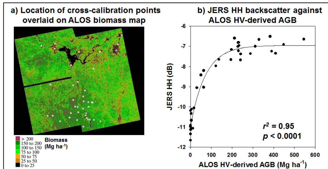
Figure 6: a) Location of 40 x 500 m x 500 m suspected unchanged areas used to back-calibrate JERS HH data to ALOS HV-derived AGB, and b) JERS HH sigma 0 from 1996 (dB) plotted against ALOS HV-derived AGB (Mg ha -1 ) from 2007 for these 40 suspected unchanged 25 ha areas.
