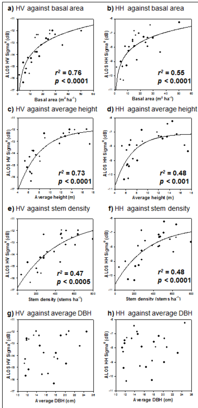
Figure 3: ALOS 2007 HV and HH sigma 0 plotted against basal area, average height, stem density and average DBH (stem diameter at 1.3 m). Best fit log relationships were fitted for a – f; no significant relationships were found for g and h.
