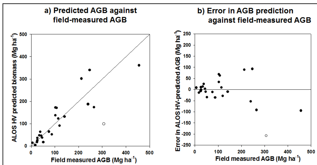
Figure 5: Errors in predicting biomass from the ALOS HV relationship are shown by a) ALOS HV-predicted AGB plotted against field-measured AGB (Mg ha -1 ), with an x = y line shown, and b) the error in ALOS HV biomass prediction plotted against field-measured biomass.
