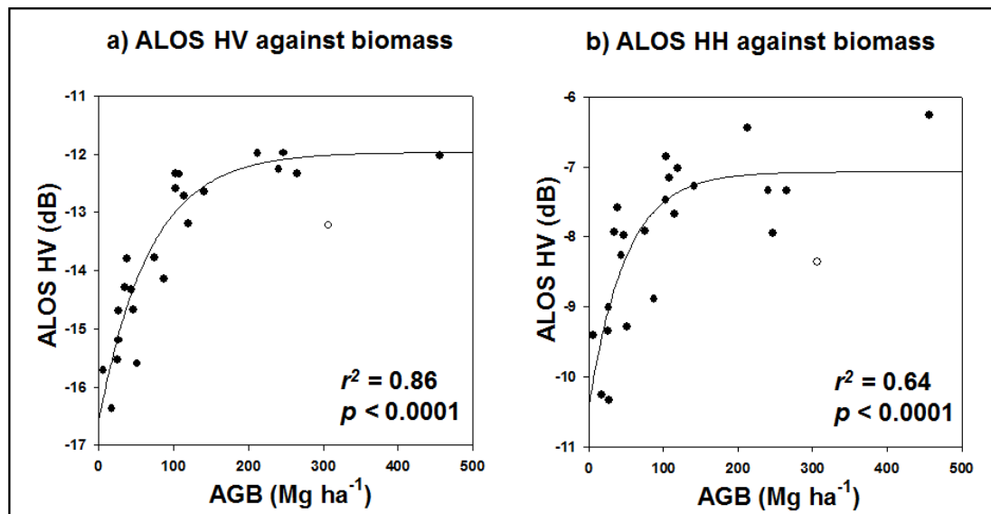
Figure 4: a) ALOS HV \sigma^0 (dB) and b) ALOS HH \sigma^0 (dB) plotted against field-measured AGB (Mg ha -1 ), with area-weighted negative exponential relationships fitted. The point in white is from a steep slope and for this reason was excluded from the regression calculations.
