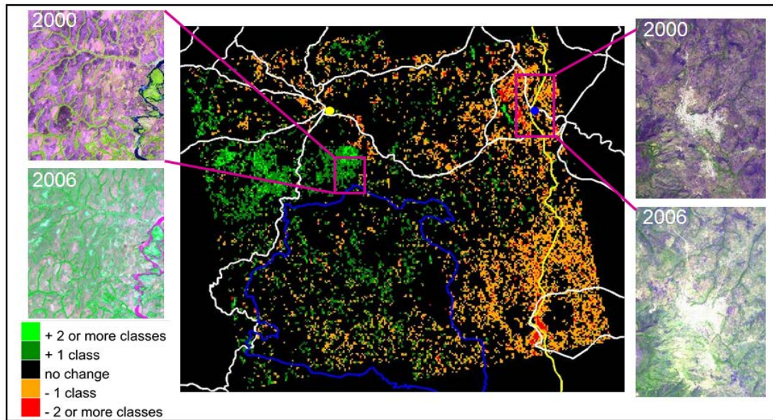
Figure 9: Change in class image using the same method as for Figure 6 c. The major towns of Tibati and Ngaundal are shown as yellow and blue circles respectively, Mbam Djerem National Park is outlined in blue, roads are shown in white, and the railway line in yellow. Optical close-up images are Landsat ETM+ from 2000 (bands 5-4-3) and ASTER from 2006 (bands 3n, 2, 1), showing the widening of gallery forests and increased woody vegetation on the left-hand pair, and the rapid clearing of woody vegetation around the town of Ngaundal on the right-hand pair. Note that the differences in color are caused by the different bands available from two sensors, however in both the green channel is an infra-red band that responds strongly to vegetation cover, which will mostly be woody in these dry season images.
