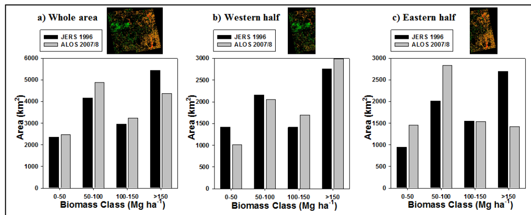
Figure 8: The total area in km 2 against biomass class (Mg ha -1 ) for the two biomass maps from 1996 and 2007 for: a) the whole data set; b) the less-populated western half of the study region; and c) the more-populated right hand half.
