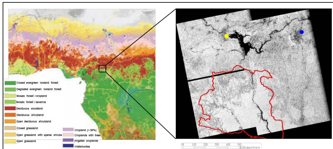
Figure 1: A section of a vegetation map of Africa taken from Mayaux et al. 2004, showing the location of the study area within Cameroon, with the ALOS HV 2007 mosaic showing the Mbam Djerem National Park outlined in red, Tibati in yellow and Ngaoundal in blue.
