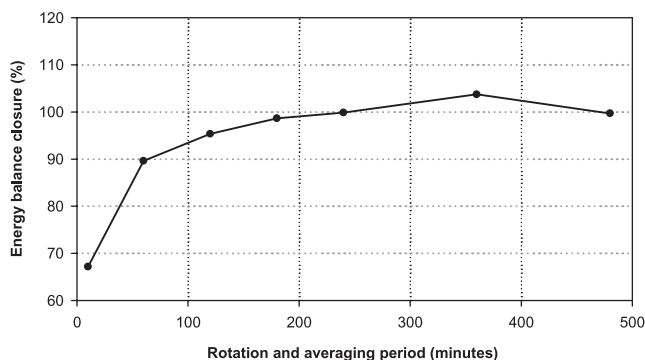
Figure 6. The variation of energy balance closure (%) with increasing rotation/averaging period (in minutes).
