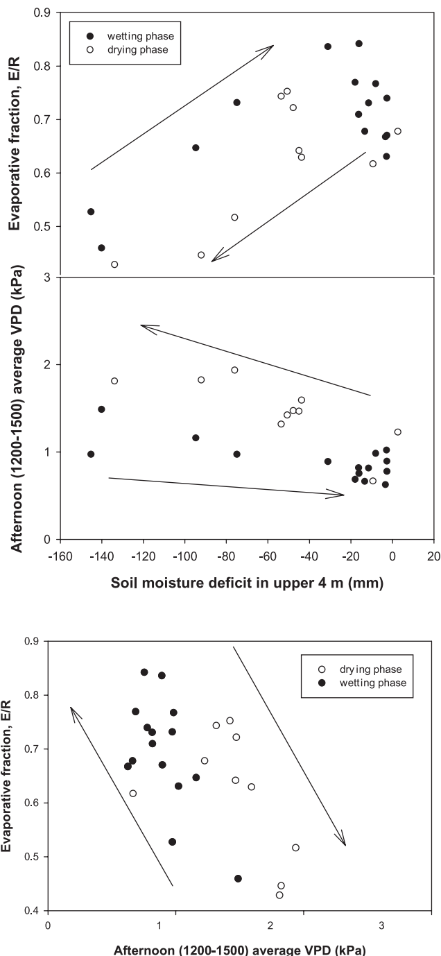
Figure 10. The relationship between (a) evaporative fraction (E/R) and soil moisture deficit, and (b) 1200–1500 water vapour pressure deficit and soil moisture deficit over the year, using 15-day averaged data. The soil moisture measurements were linearly interpolated to the middle of each 15-day period. Open circles indicate the drying phase of the seasonal cycle (soil moisture decreasing), and solid circles the wetting phase.
