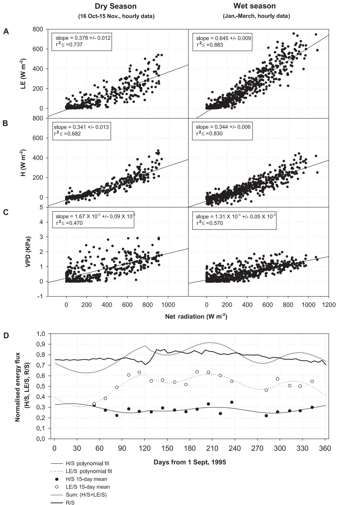
Figure 5. The relationships between (a) the turbulent latent heat flux, LE, and net radiation, R; (b) the turbulent sensible heat flux, H, and net radiation, R; (c) the atmospheric water vapour pressure deficit (VPD) and R. (d) 15-day values of H, LE, (H + LE), and R, calculated from plots of the variable against incoming solar radiation S. Note that (H + LE) is close to R for much of the year.
