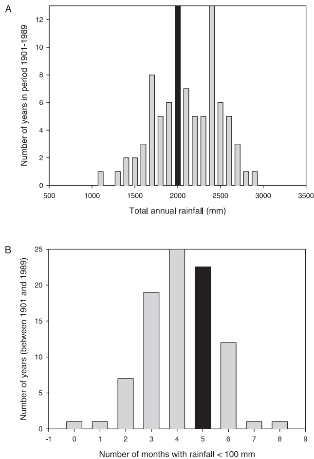
Figure 2. Frequency distribution of (a) rainfall and (b) number of dry months in the nearby city of Manaus between 1901 and 1989 (excluding 1909, when data were collected). The value for the measurement period (September 1995 to August 1996) is shown in black. A dry month is defined as having rainfall <100 mm.
