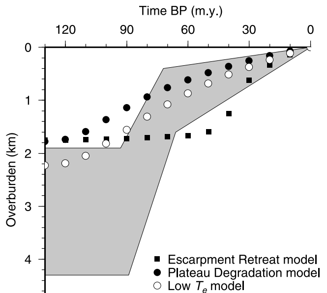
Figure 6. Denudation history for a point located 30 km seaward of the escarpment for the models shown in Figure 5. Plot shows the (strike-averaged) overburden for points now at the surface as a function of time before present. Shaded polygon represents spectrum of acceptable denudation histories from the Swartberg well fission track data [cf. Brown et al. , 2002] for comparison with model predictions.
