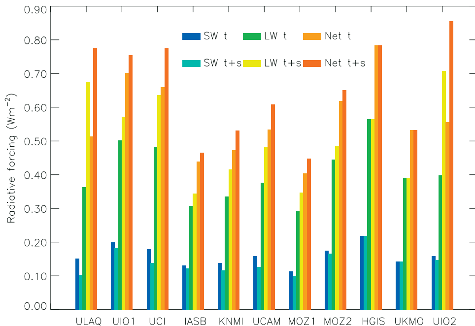
Figure 9. Components of global-mean radiative forcing for each model ( W m^{-2} ). SW, shortwave component; LW, longwave component; t, including tropospheric ozone changes only; and t + s, including both tropospheric and stratospheric changes. (Note: for ULAQ and UIO2 the t + s bars refer to the experiments calculating stratospheric ozone change discussed in section 2.2.)
