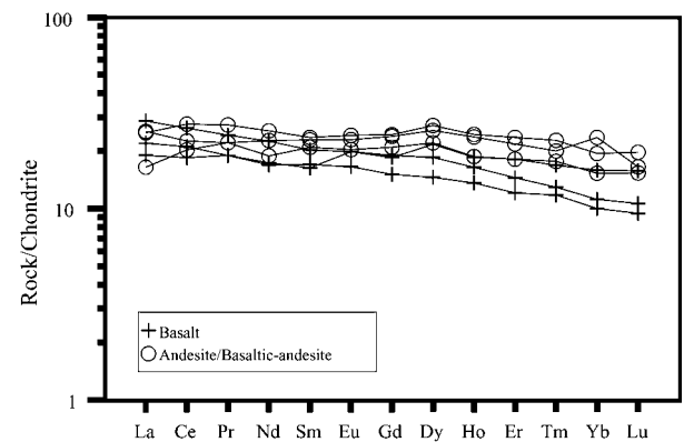
Figure 11. Chondrite-normalized REE patterns of volcanic rocks from the Mersin Melange (normalizing values from Sun & McDonough, 1989).
