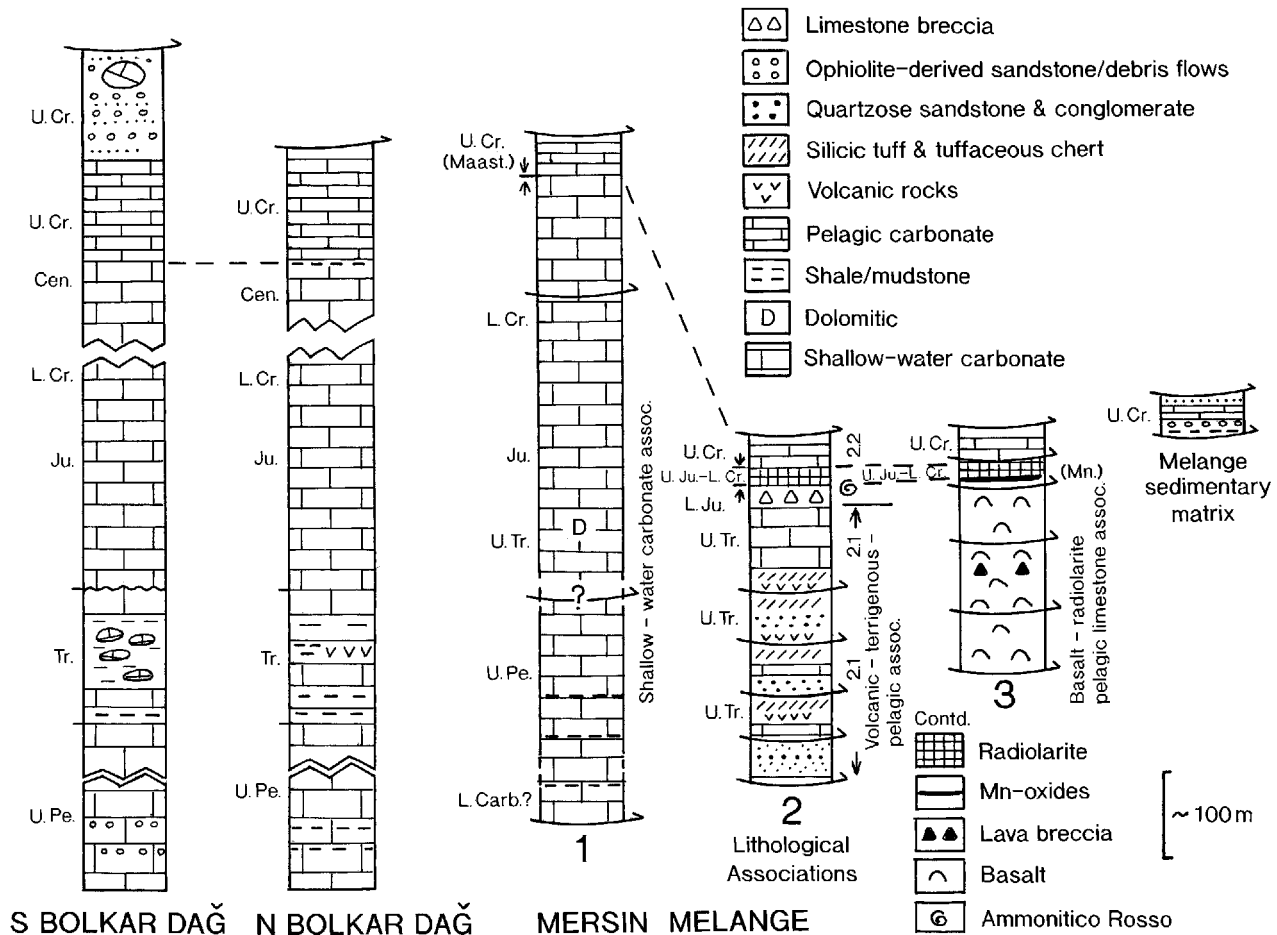
Figure 6. Generalized logs of the main lithological units exposed in the Bolkar Dağ (Northern and Southern units) and the Mersin Melange. The columns 1–3 are for the Mersin Melange, as follows: (1) shallow-water carbonate association; (2) volcanic–terrigenous–pelagic association; (3) basalt radiolarite–pelagic limestone association.
