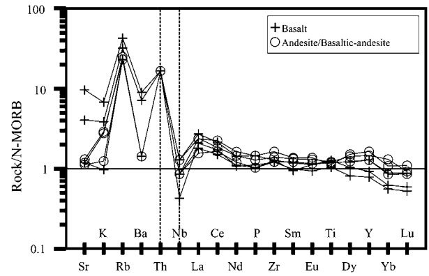
Figure 10. N-MORB normalized multi-element diagram for volcanic rocks from the Mersin Melange (normalizing values from Sun & McDonough, 1989).
