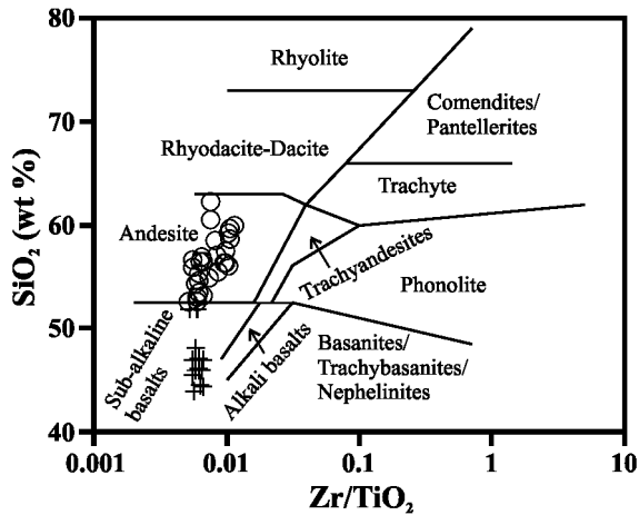
Figure 9. Discrimination of different volcanic rock types in the Mersin Melange based on \text{SiO}_2 vs. \text{Zr}/\text{TiO}_2 (after Floyd & Winchester, 1978).
