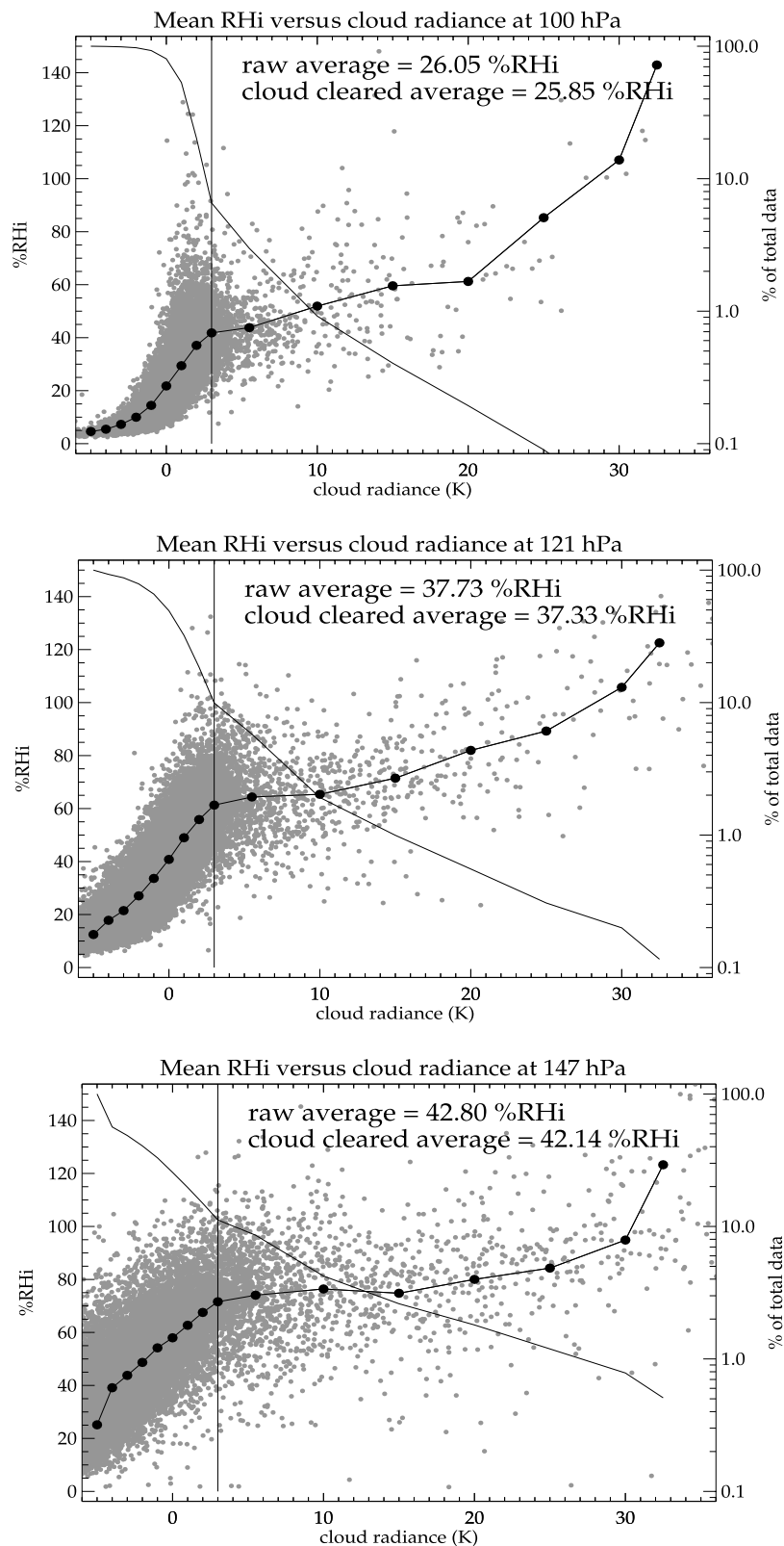
Figure 3. Scatterplots of cloud radiance versus V7.02 H 2 O in %RH i at (top) 100 hPa, (center) 121 hPa, and (bottom) 147 hPa. The line with bullets is average %RH i as a function of cloud radiance. The plain line is (right y-axis) percentage of measurements having cloud radiances equal or greater than that given by the x-axis. The data are from January to March 1992, 25°S to 25°N. Cloud radiance >3 K indicates high probability of a cloud in the MLS field-of-view.
