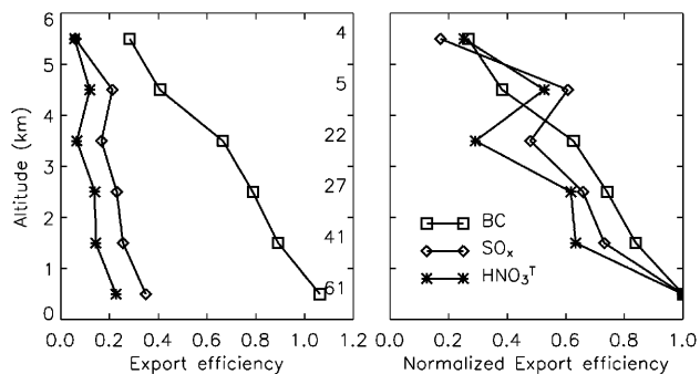
Figure 1. Mean vertical profiles of (left) export efficiency and (right) normalized export efficiency in Asian outflow for black carbon (BC) (squares), \text{SO}_x defined as the sum of \text{SO}_2 and fine non-sea-salt sulfate aerosol (diamonds), and \text{HNO}_3^T defined as the sum of \text{HNO}_3 and fine inorganic nitrate aerosol (asterisks). The export efficiencies are derived by application of equations (1) and (2) to the Transport and Chemical Evolution over the Pacific (TRACE-P) P-3B measurements over the NW Pacific ( 30^\circ\text{--}41^\circ\text{N} , 124^\circ\text{--}140^\circ\text{E} ). The number of measurements used to calculate export efficiencies at each altitude is also shown.
