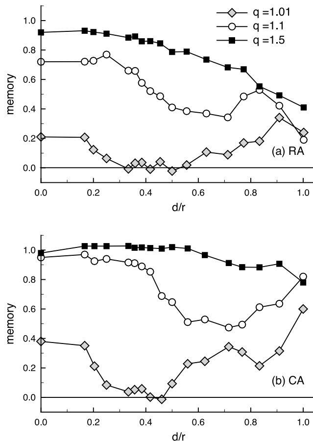
Figure 8. Magnetic memory ratio ( \text{MR} ) versus d/r for (a) the RA model and (b) the CA model for three effective elongations, i.e., q = 1.01, 1.1 and 1.5. As d/r increases the spacing between grains decreases. The uniaxial anisotropy is chosen randomly compared to the crystal morphology.
