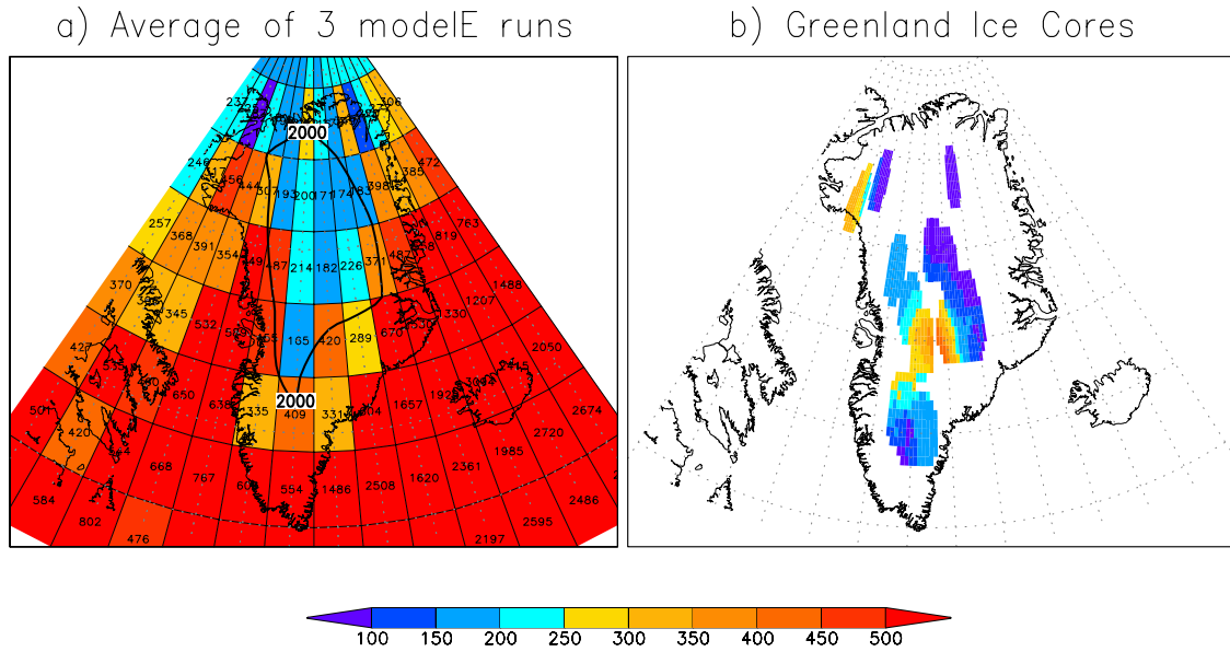
Figure 7. (a) Total SO 4 (kg/km 2 ) deposition from the Laki eruption to Greenland and surrounding areas averaged from the three simulations. The 2000 m elevation is shown on Greenland. (b) Total SO 4 (kg/km 2 ) deposition from 23 Greenland ice cores (C. Gao et al., manuscript submitted to Journal of Geophysical Research , 2006).
