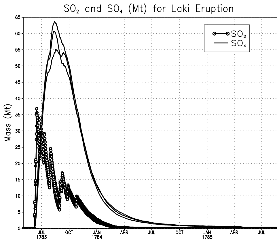
Figure 5. Daily mass loading of \text{SO}_2 and \text{SO}_4 (Mt) for the three simulations of the Laki eruption with the background loadings removed. The Laki simulations are from May 1783 through August 1785.
