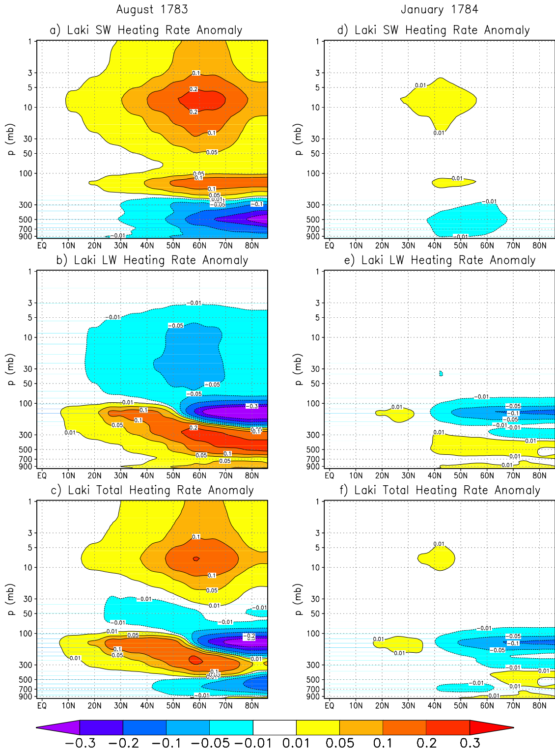
Figure 11. Zonal mean monthly averaged heating rate anomalies (K/day) for August 1783 (left column) and January 1784 (right column) from the surface to 1 mbar for the Northern Hemisphere. Shown are shortwave heating rate anomalies (Figures 11a and 11d), longwave heating rate anomalies (Figures 11b and 11e), and total heating rate anomalies (Figures 11c and 11f).
