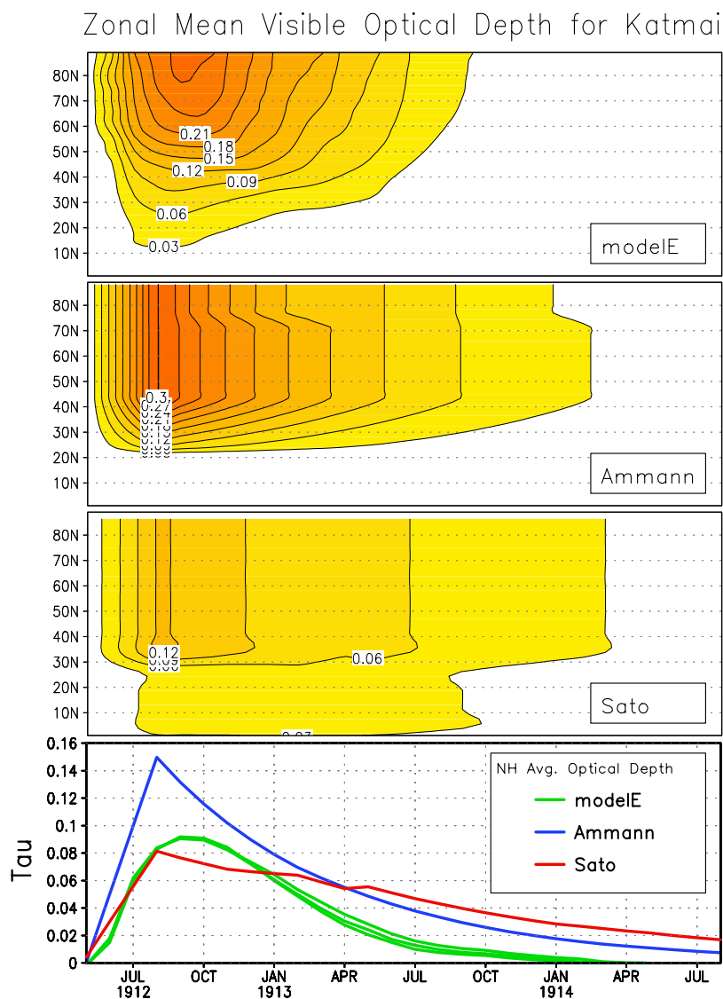
Figure 4. Zonal mean sulfate optical depth for Katmai from three modelE simulations, compared to Ammann et al. [2003] and Sato et al. [1993] data with backgrounds removed. The bottom panel is Northern Hemisphere average optical depth for the three individual modelE runs, Ammann et al. [2003], and Sato et al. [1993]. The optical depths are from May 1912 through August 1914.
