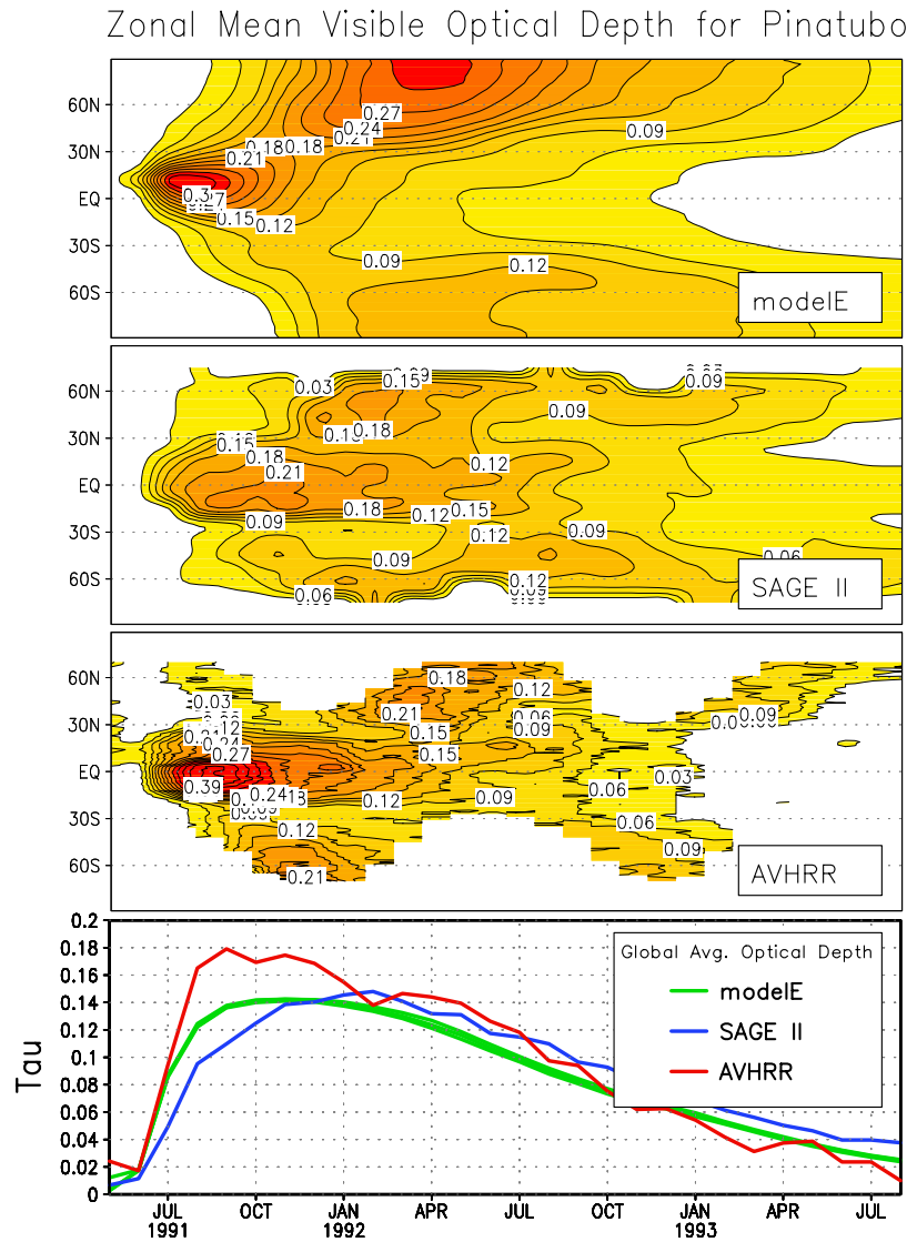
Figure 3. Zonal mean sulfate optical depth for Pinatubo from three modelE simulations, compared to SAGE II and AVHRR data with backgrounds removed. The bottom panel is global average optical depth for the three individual modelE runs, SAGE II, and AVHRR. The optical depths are from May 1991 through August 1993.
