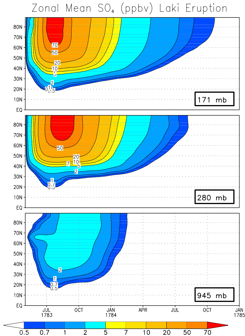
Figure 9. Zonal mean SO 4 concentrations (ppbv) for the Laki eruption over the Northern Hemisphere from May 1783 through January 1785 for (top) 171 mbar, (middle) 280 mbar, and (bottom) 945 mbar.
