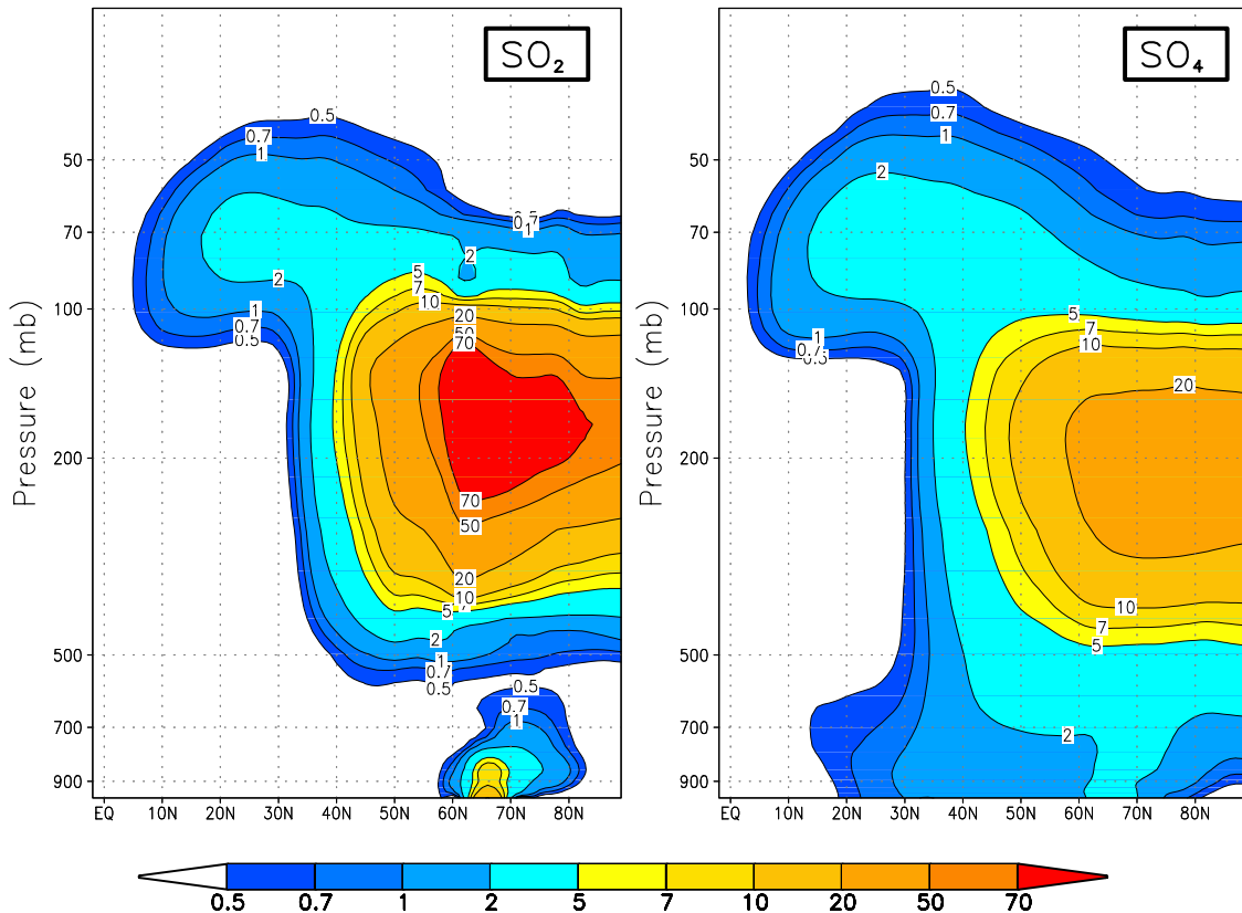
Figure 8. The 30°W to 45°E mean (left) SO 2 and (right) SO 4 concentrations (ppbv) for June–August 1783 over the Northern Hemisphere from the surface to 30 mbar.
