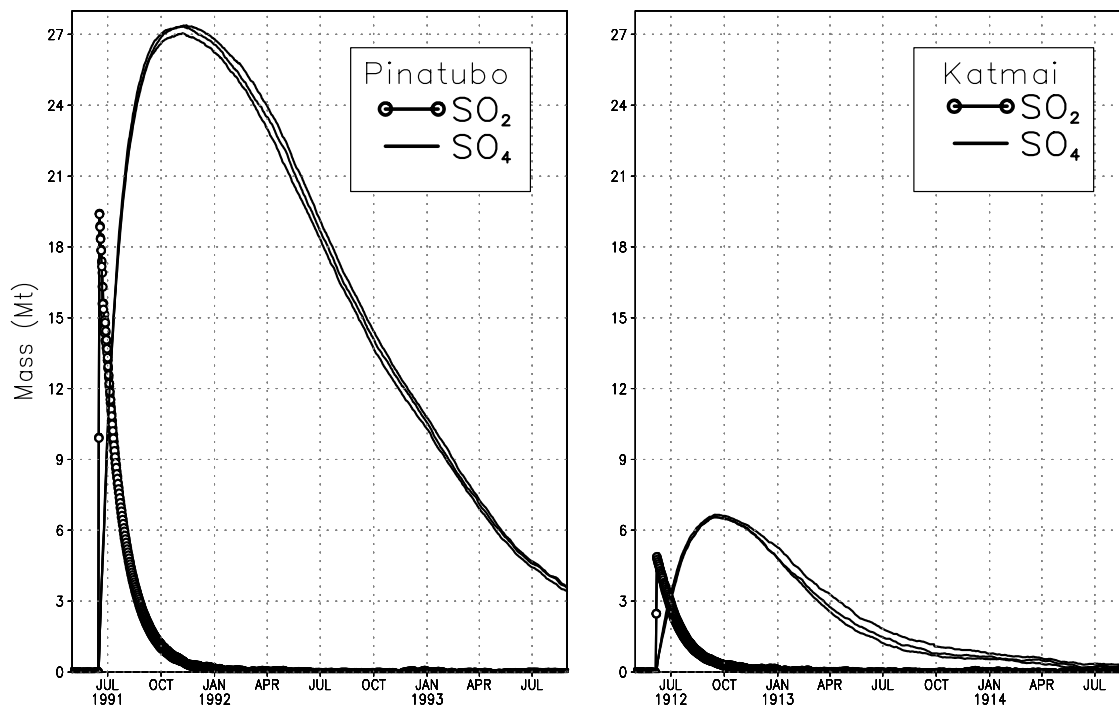
Figure 2. Daily mass loading of SO 2 and SO 4 (Mt) for the three simulations of (left) Pinatubo and (right) Katmai with the background loadings removed. The Pinatubo simulations are from May 1991 through August 1993. The Katmai simulations are from May 1912 through August 1914.
