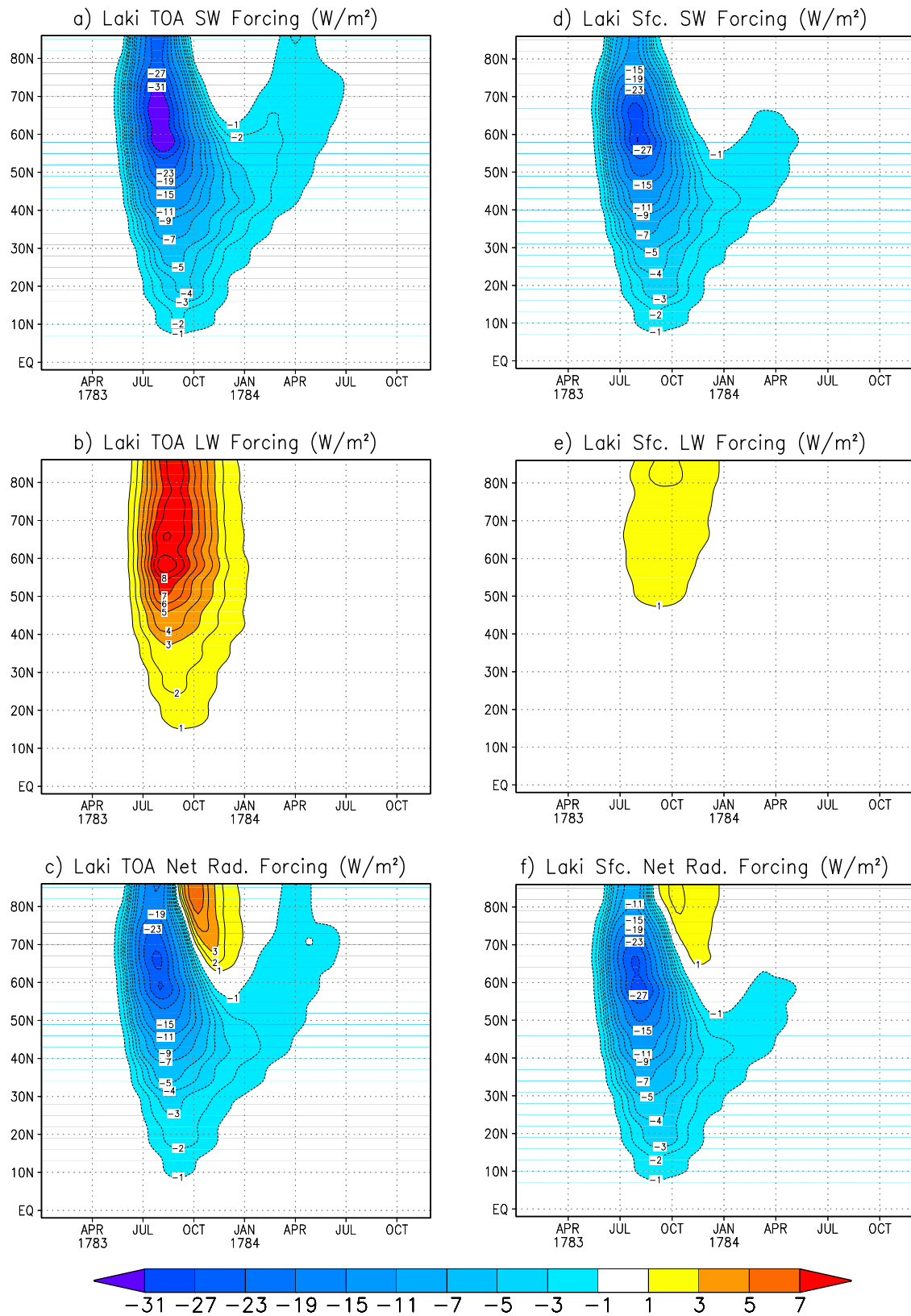
Figure 10. All-sky radiative forcings ( W/m^2 ) calculated for the Laki eruption from January 1783 through December 1784 for the Northern Hemisphere. Shown on the left are (a) TOA shortwave forcing and (b) TOA longwave forcing, as well as (c) TOA net radiative forcing. Shown on the right are (d) surface shortwave forcing and (e) surface longwave forcing, as well as (f) surface net radiative forcing.
