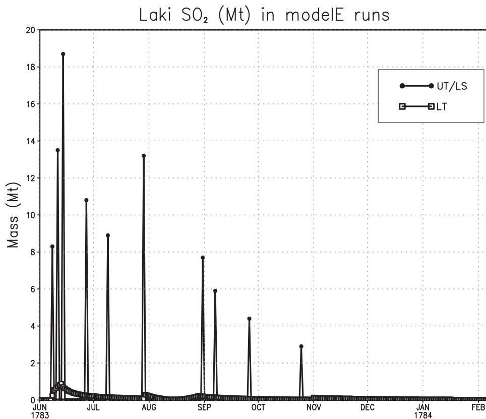
Figure 1. Daily mass of \text{SO}_2 gas (Mt) for Laki eruption used in modelE runs from 1 June 1783 to 7 February 1784, based on Figure 2 from Thordarson and Self [2003]. The lower troposphere (LT) injection is shown as a line with open squares, and the upper troposphere/lower stratosphere (UT/LS) is shown as a line with solid circles.
