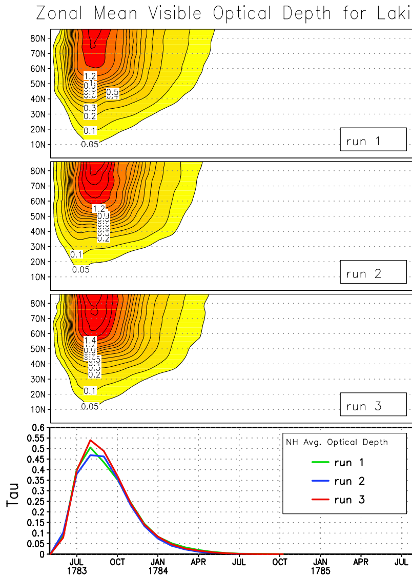
Figure 6. Zonal mean sulfate optical depth for Laki from three modelE simulations with backgrounds removed. The bottom panel is Northern Hemisphere average optical depth for the three individual modelE runs. The optical depths are from May 1783 through August 1785.
