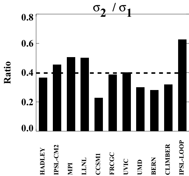
Fig. 3. Ratio of the standard deviations ( SD ) in \Delta T_{2100} (K) for each baseline C4MIP model replicated by HadSCCM1, due to variations in carbon cycle parameters ( \sigma_2 , i.e. SD of green values for each model in Fig. 1) and variations in physical climate parameters ( \sigma_1 , i.e. SD of red values for each model in Fig. 1). The horizontal dashed line is the mean value of these ratios.
