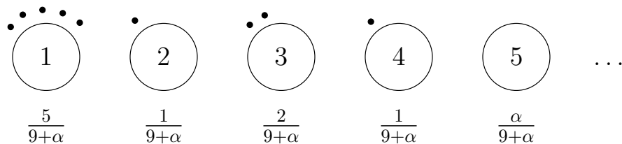
Figure 9: The Chinese restaurant process. Black dots indicate the seating arrangement of the first nine customers. Below each table is P(z_{10} = k | \mathbf{z}_{-10}) .
