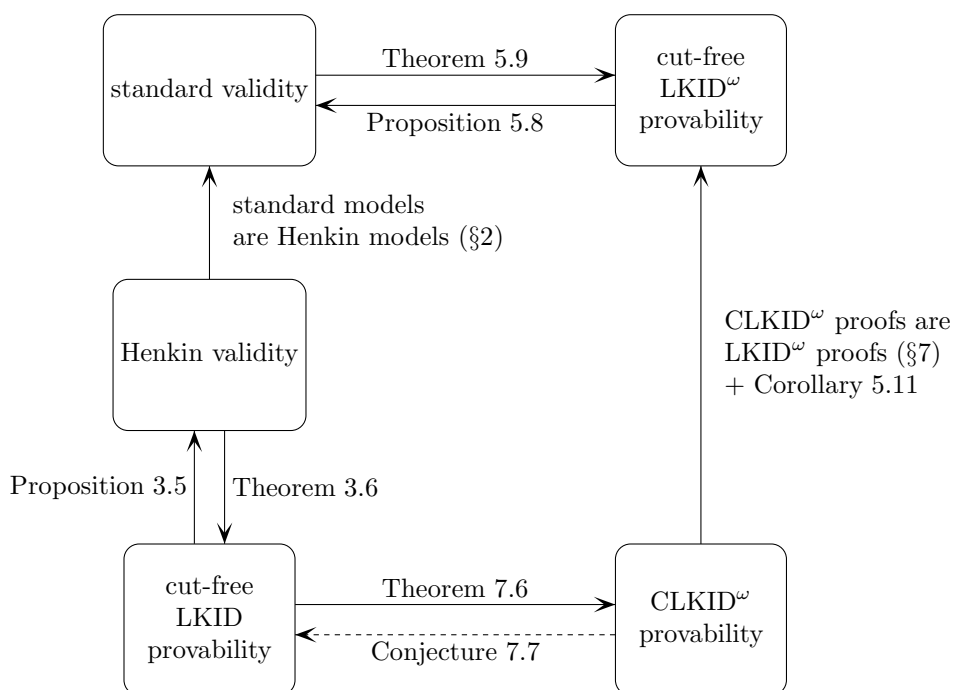
Figure 5: A diagrammatic summary of our developments. The solid arrows are implications, and the dashed arrow indicates our conjectured implication.
