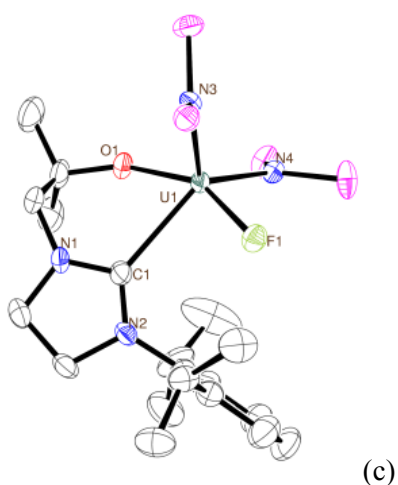
Figure 1. Displacement ellipsoid drawings of the molecular structures of a) [\text{Ce}(\text{L})(\text{N}'')_2\text{Cl}] , b) [\text{U}(\text{L})(\text{N}'')_2\text{Cl}] , and c) [\text{U}(\text{L})(\text{N}'')_2\text{F}] . Lattice solvent molecules, hydrogen atoms and silyl methyl groups are omitted for clarity.
