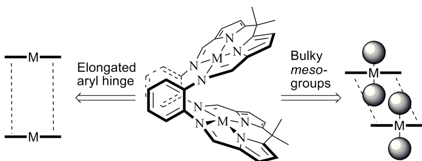
Chart 1. Ligand design strategies to disfavour single-atom-bridged binuclear complexes.
