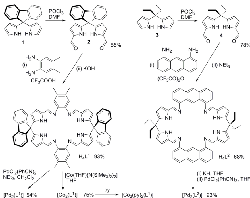
Scheme 1. The synthesis of the fluorenyl and anthracenyl Schiff-base calixpyrroles H 4 L 1 and H 4 L 2 and their binuclear Pd and Co complexes
