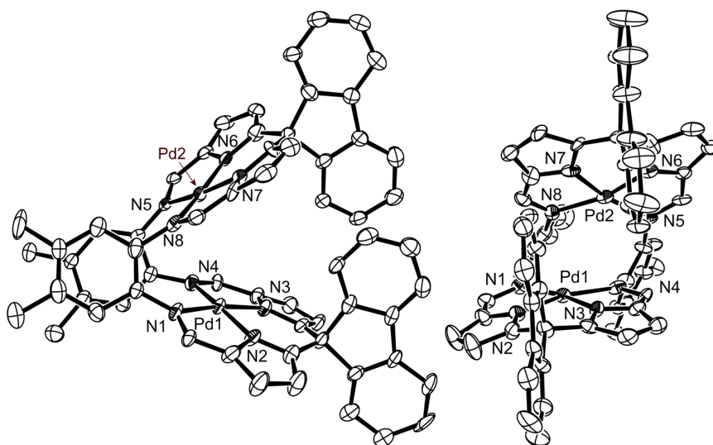
Figure 2. Solid state structure of [Pd 2 (L 1 )](Et 2 O) 2.5 (left: side-on; right: face-on). For clarity, all hydrogen atoms and solvent of crystallisation are omitted (displacement ellipsoids are drawn at 50% probability).
