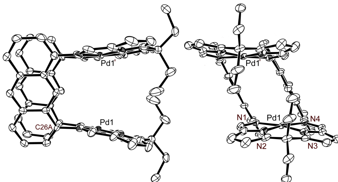
Figure 4. Solid state structure of [\text{Pd}_2(\text{L}^2)](\text{NEt}_3)(\text{CDCl}_3) (Left: side-on view; right: face on view). For clarity, all hydrogen atoms and solvents of crystallisation are omitted (displacement ellipsoids are drawn at 50% probability). The two palladium atoms Pd1 and Pd1' are related by the symmetry operation -x, y, \frac{1}{2}-z .
