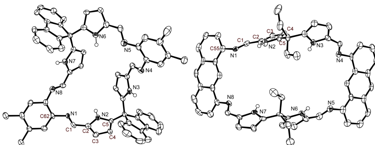
Figure 1. X-ray crystal structures of H 4 L 1 (CH 2 Cl 2 ) 2 (left) and H 4 L 2 (CH 2 Cl 2 )(MeOH) 3.25 (right). For clarity, all hydrogen atoms, except those bound to the pyrrolic nitrogens, and solvent of crystallisation are omitted (displacement ellipsoids are drawn at 50% probability).
