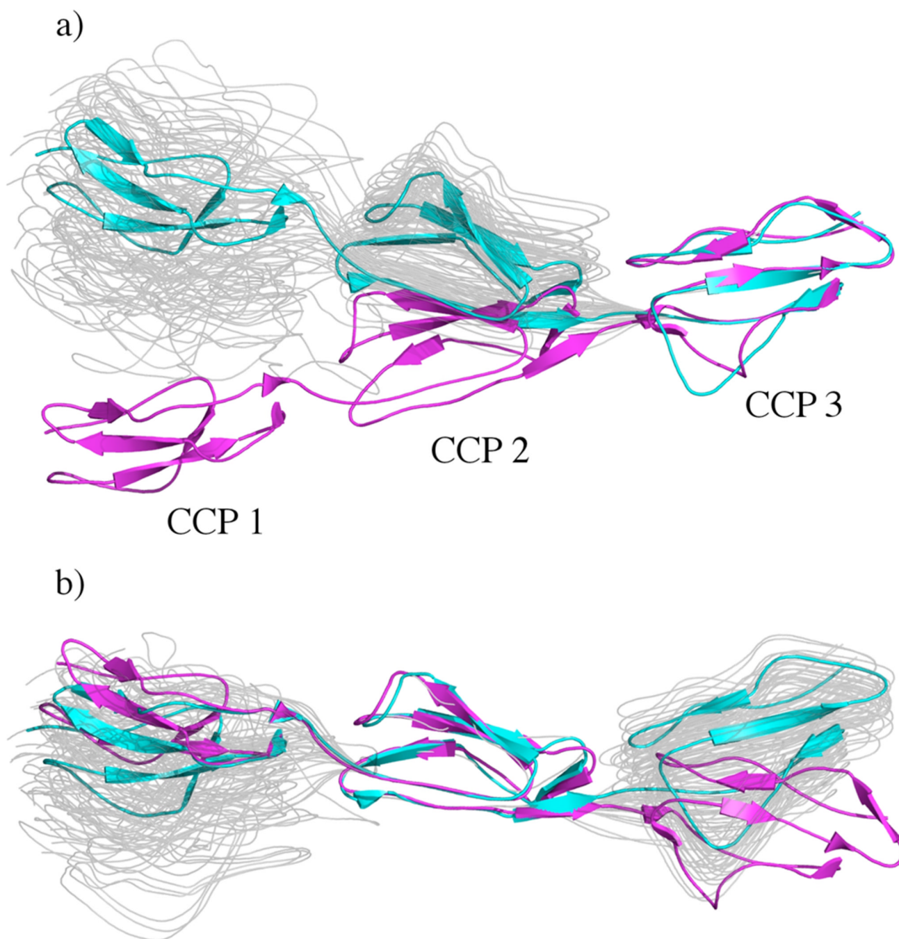
Figure 6. CCPs 1–3 of FH in crystal structure (magenta), lowest-energy NOE/RDC refined structure (cyan) and structural ensembles within the 40° cone representing flexional freedom (grey). a) Least square fit on CCP 3 of the crystal structure. b) Least square fit on CCP 2 of the crystal structure. None of the solution structures reproduces the crystal structure conformation.
