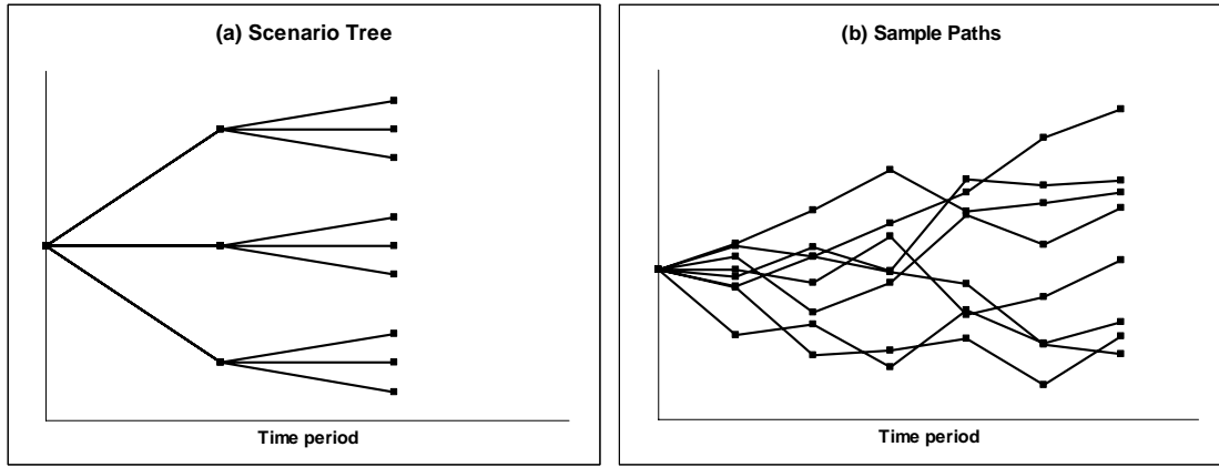
Figure 1: Scenario Generation
