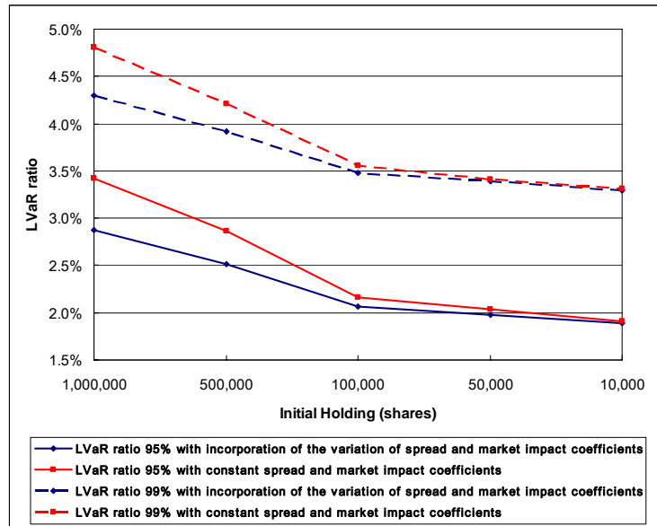
Figure 3: LVaR ratio comparison
