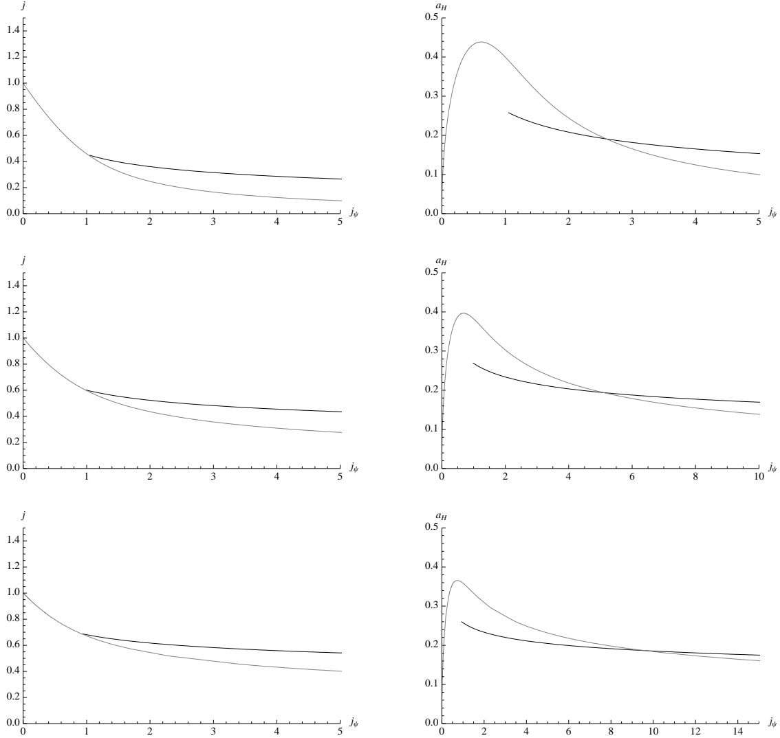
Fig. 6: Phase diagram for extremal black holes and black rings with equal angular momenta on the transverse S^{2n} in D = 7, 9, 11 (in this order.) In all cases, the gray curve corresponds to the MP black hole and the black one to the black ring. The corresponding phase diagram for D = 5 is given in Fig. 5. The ring curve is terminated at the point of intersection with the MP curve; this preserves uniqueness and provides a lower bound on the allowed value of j_\psi . Left: Plot of the j vs. j_\psi curve, where j = j_i is any of the angular momenta on the S^{2n} . Right: Plot of the a_H vs. j_\psi curve.
