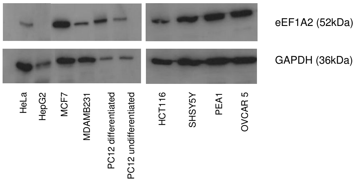
Figure 1 Western blot analysis using an anti-eEF1A2 antibody on a range of cell lines. The loading control is GAPDH.
