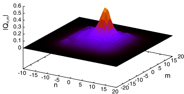
FIG. 6 (color online). Solution of 2 + 1 dimensional DNLS equation (2) for |Q_{m,n}| at z = 10 for the initial conditions a = 1.5 , w = 1.5 , and V = 0.25 with \mu = 1.4 and q = 0.18 .
