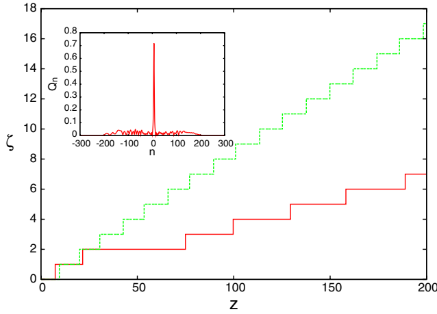
FIG. 2 (color online). Position \zeta of the soliton from the DNLS equation (1) for the initial conditions a = 0.7 , w = 1.5 , and V = 0.1 with q = 0.15 and \mu = 0.8 . Numerical solution: solid line (red); solution of modulation equations: dashed line (green). The inset shows the solution for |Q_n| at z = 200 .
