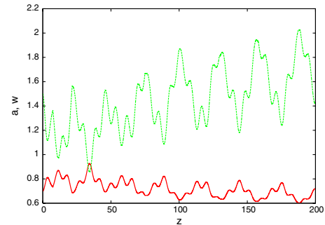
FIG. 1 (color online). Solution of DNLS equation (1) for the amplitude a (solid line, red) and width w (dashed line, green) of the solitary wave as given by the numerical solution for the initial conditions a = 0.7 , w = 1.5 , and V = 0.1 with q = 0.15 and \mu = 0.55 .
