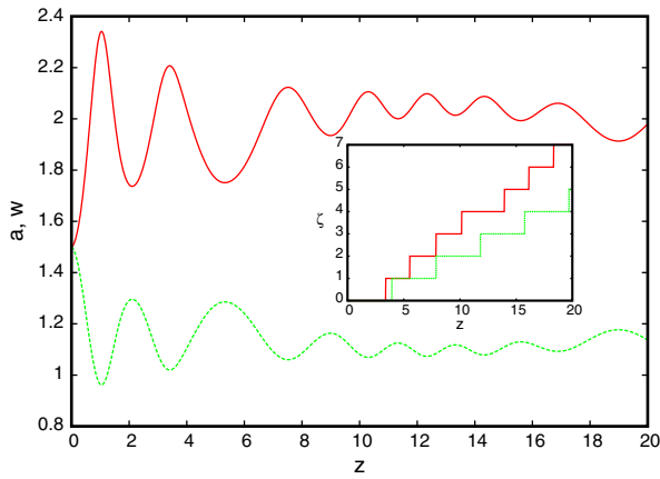
FIG. 5 (color online). Solution of 2 + 1 dimensional DNLS equation (2) for the initial conditions a = 1.5 , w = 1.5 , and V = 0.25 with q = 0.18 . Numerical amplitude a (solid line, red) and width w (dashed line, green) for \mu = 0.5 . Inset: position \zeta for \mu = 1.4 . Numerical solution: solid line (red); solution of modulation equations: dashed line (green).
