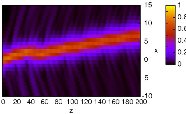
FIG. 3 (color online). Evolution in xz of the solution of the DNLS equations (1) for the initial conditions a = 0.7 , w = 1.5 , and V = 0.1 with q = 0.15 and \mu = 0.8 .
