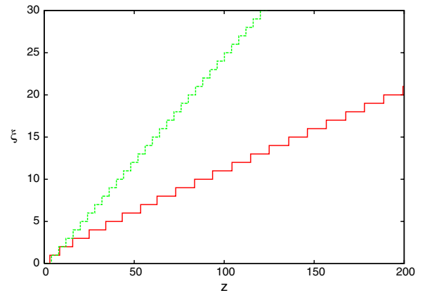
FIG. 4 (color online). Position \zeta for the DNLS equation (1) for the initial conditions a = 0.7 , w = 1.5 , and V = 0.25 with q = 0.15 and \mu = 0.38 . Numerical: solid line (red); modulation: dashed line (green).
