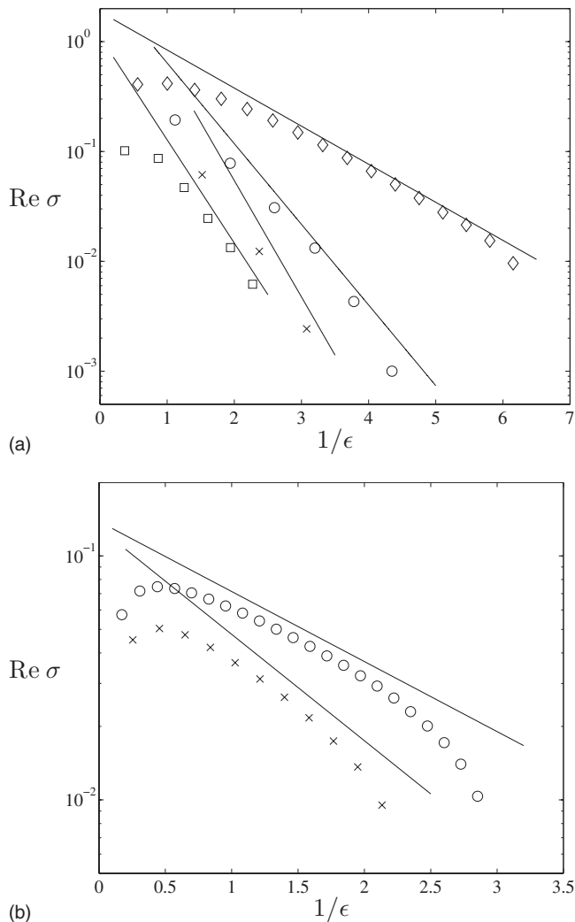
FIG. 2. Numerical estimates of the local maxima of the growth rates \text{Re } \sigma as functions of the inverse Rossby number 1/\epsilon . (a) Anticyclonic flows with e=1.5 , \mu=1 ( \times ); e=2 , \mu=1 ( \circ ); e=2 , \mu=0.5 ( \square ); and e=4 , \mu=1 ( \diamond ). (b) Cyclonic flows with e=4 , \mu=0.5 ( \times ); and e=6 , \mu=0.5 ( \circ ). The straight lines in these linear-logarithmic plots indicate the exponential dependence predicted by asymptotic estimate (3.11).
