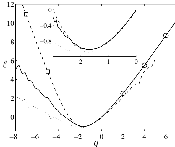
FIG. 4. Generalised Lyapunov exponents of the product of the random matrices (51) with a = b = c = \pi . The RMC estimates of \ell(q) obtained for N = 100 with an ensemble size K = 1000 (solid line) and K = 100 (dotted line) are compared with an estimate of \ell^-(-q - 3) obtained by applying the RMC method to A^{-1} with K = 1000 (dashed line). The results of the replica method, applied to A (circles) and A^{-1} (squares) are also indicated. The curves in the inset, which displays a close up of the region -3 \leq q \leq 0 , have been computed using K = 5000 .
