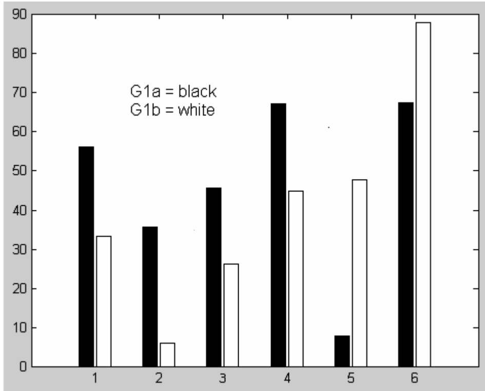
Figure 14: Co-plot of first six elements of vectors G1a centroid and G1b centroid
