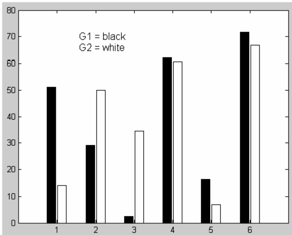
Figure 13: Co-plot of first six elements of vectors G1_{\text{centroid}} and G2_{\text{centroid}}
