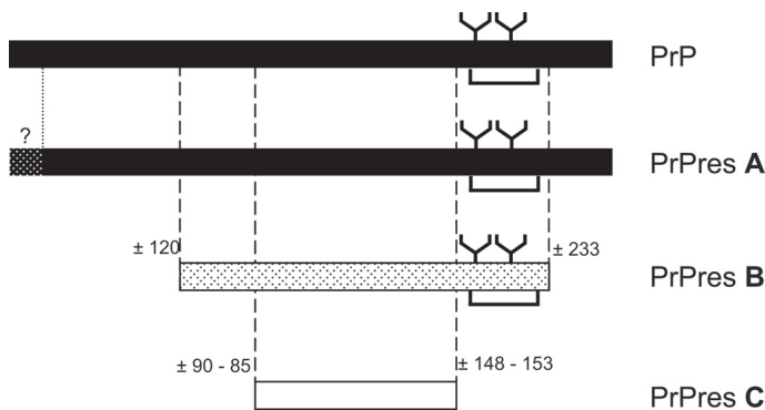
Figure 3. Line diagram illustrating the fragmentation of the atypical/Nor98 PrP.
