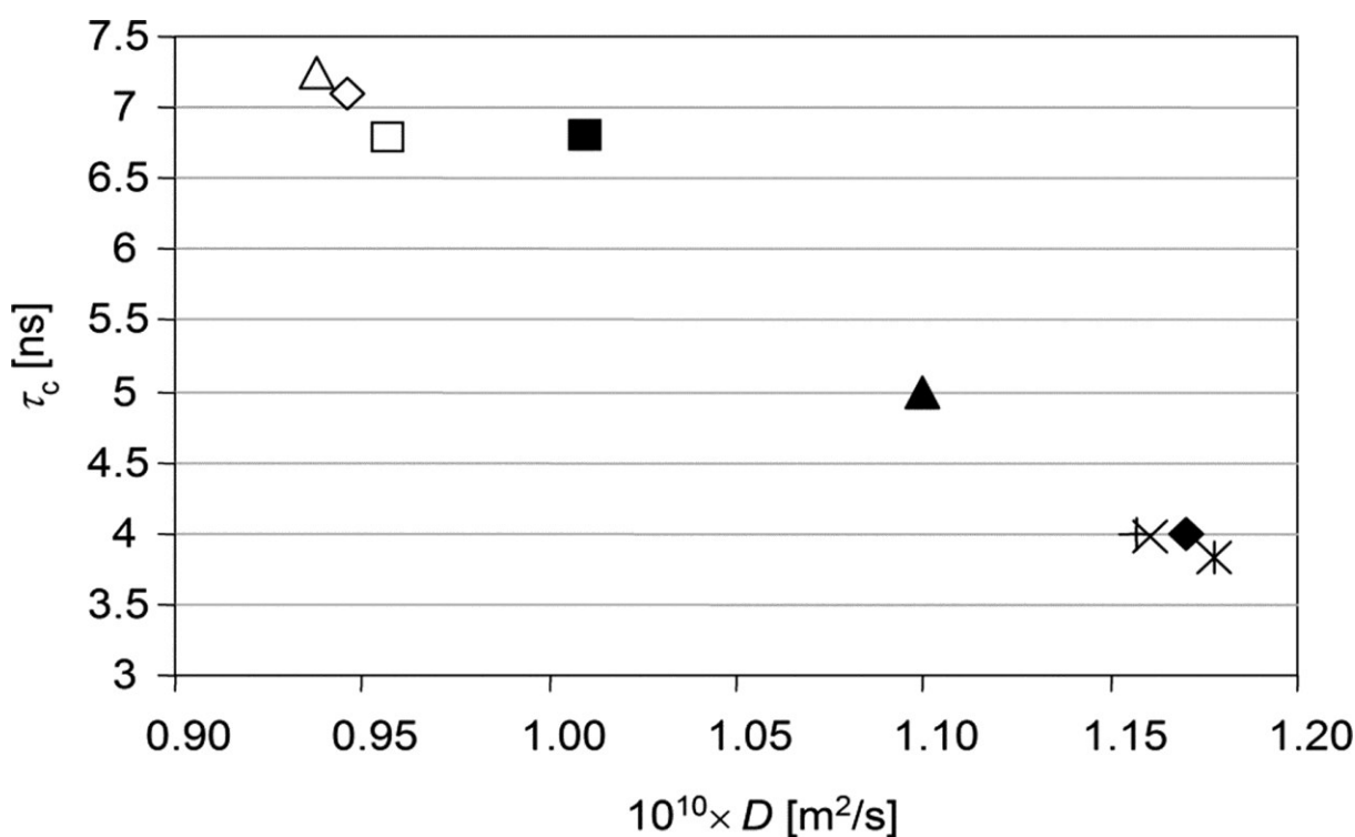
Figure 8. Plot of experimental (♦) and theoretical (*, AER 2.3 Å), (×, AER 2.4 Å), and (+, AER 2.5 Å) rotational correlation times, \tau_c , vs diffusion coefficients, D , for monomeric HBD2. Theoretical values for an HBD2 dimer (pdb entry 1FD3) are shown using □ (AER 2.3 Å), ◇ (AER 2.4 Å) and △ (AER 2.5 Å). Experimental values for the GAG/HBD2 mixtures are displayed as ■ (FX/HBD2 16:1) and ▲ (DS-dp6/HBD2 4:1).
