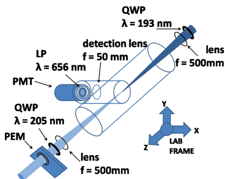
FIG. 2. Schematic for the experimental setup (PEM, photoelastic modulator; QWP, quarter-wave plate; LP, linear polarizer; and PMT, photomultiplier tube).
