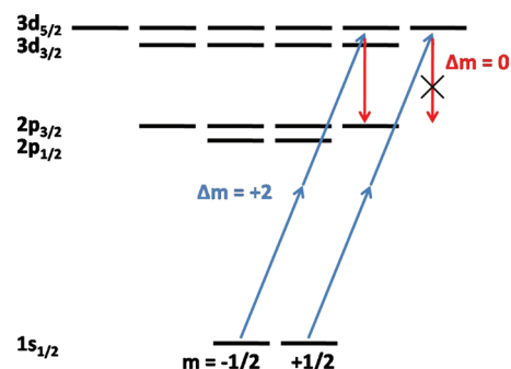
FIG. 1. The polarization-sensitive LIF detection scheme. Absorption of two circularly polarized photons and detection of linearly polarized fluorescence leads to complete m -state selectivity in the H-atom detection.
