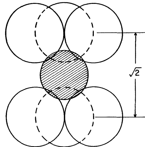
STRETCHED TRIGONAL PRISM 0.8257
