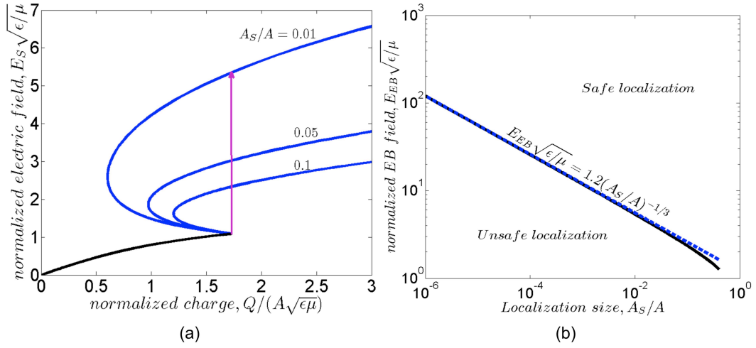
FIG. 4. Electromechanical localization and electrical breakdown. (a) Bifurcation diagram plotted on the plane of the total charge Q and the electric field in the small part E_S . (b) The condition under which electromechanical localization does not cause electrical breakdown.
