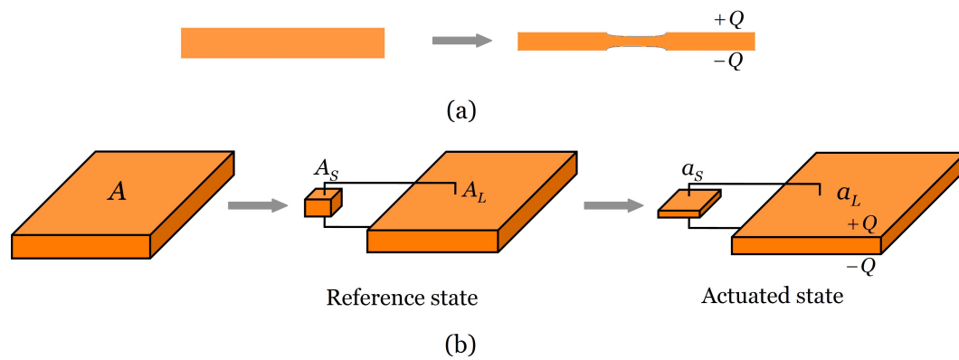
FIG. 2. Localized deformation. (a) When the membrane with compliant electrodes is charged beyond a critical value, the homogeneous deformation is unstable, and a small region of the membrane deforms more than the rest of the membrane. (b) A model of localization represents the membrane by two regions subject to the same voltage, but each region undergoes a separate homogeneous deformation.
